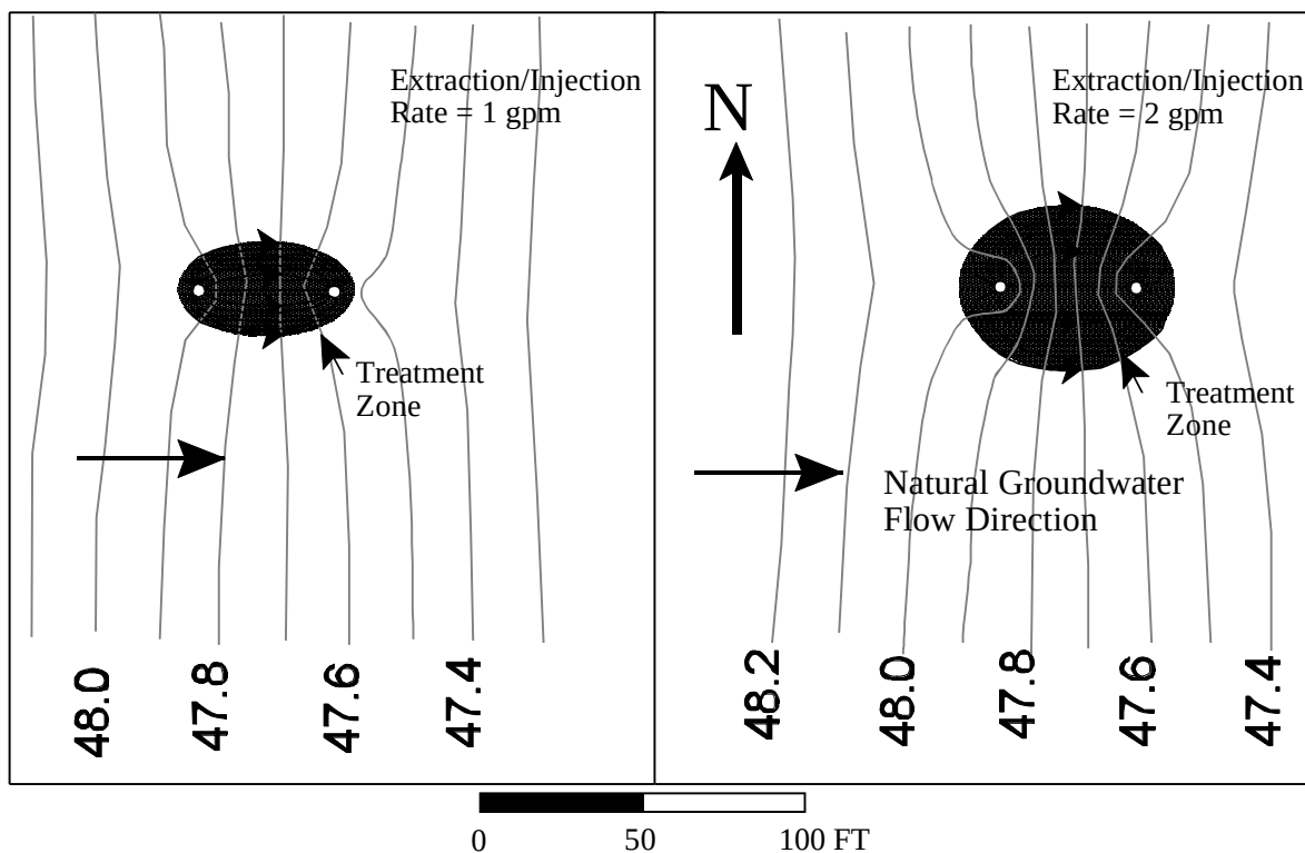
Figure 10. Hydrogeologic modeling results showing the effects of increasing extraction/injection rate. Model is for unconfined flow in a uniform aquifer 100 feet thick with hydraulic conductivity of 0.005 cm/s. Boundary conditions include constant heads on the east and west margins.
