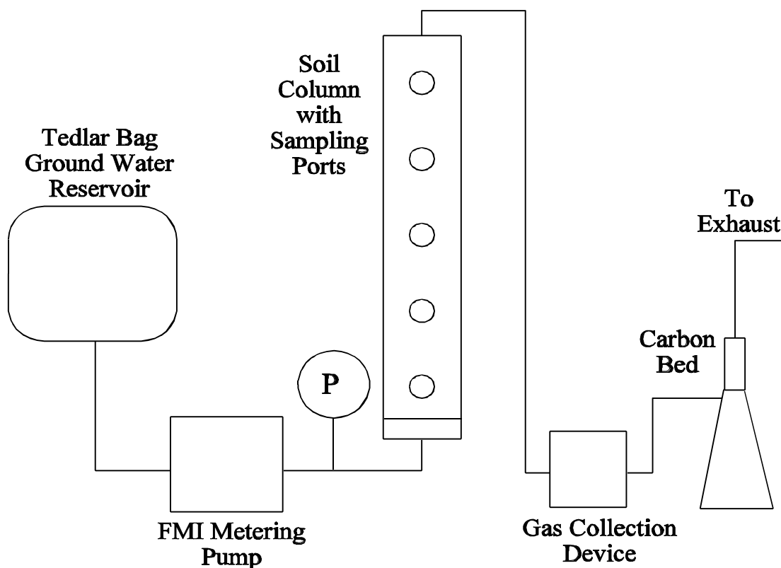
Figure 8. Schematic of soil column set-up. Modified from Harkness et al. (1998).
