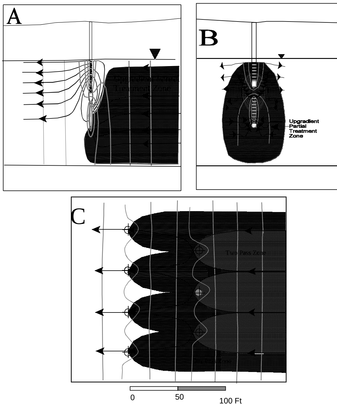
Figure 13. Hydrogeologic model of vertical recirculating well. A) is a cross section oriented parallel to groundwater flow. Groundwater enters in a lower screen and exits from an upper screen. B) is a cross section perpendicular to flow. It shows the width of the upgradient partial treatment zone. C) is a map showing two rows of vertical recirculation wells, as well as upgradient treatment zone with a minimum of one pass (lighter) and two passes (darker).
