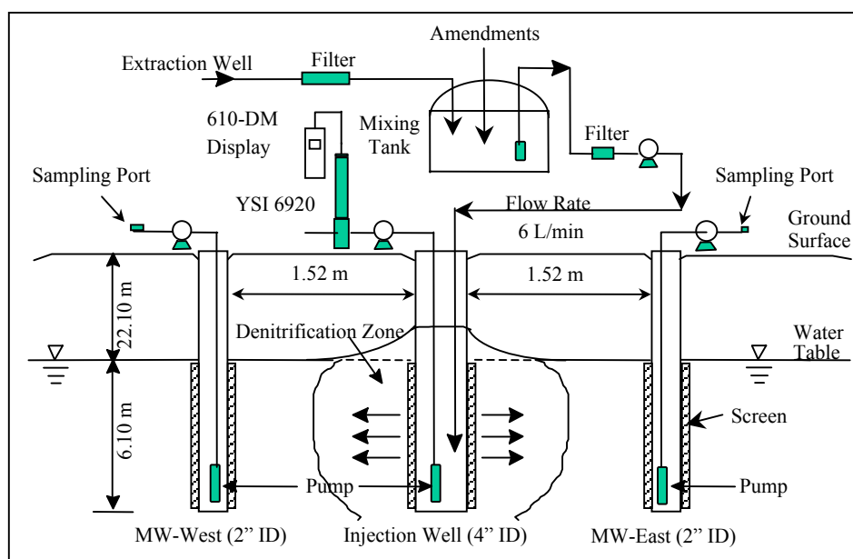
Figure 8-3. Design of an In Situ Denitrification Test at Tri-Tech Site, Albuquerque's South Valley (not drawn to scale)
