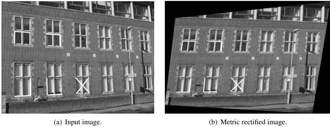
Figure 7: Building metric upgrade. The perspective effect of the original image is removed using orthogonal properties of the facade structure.
