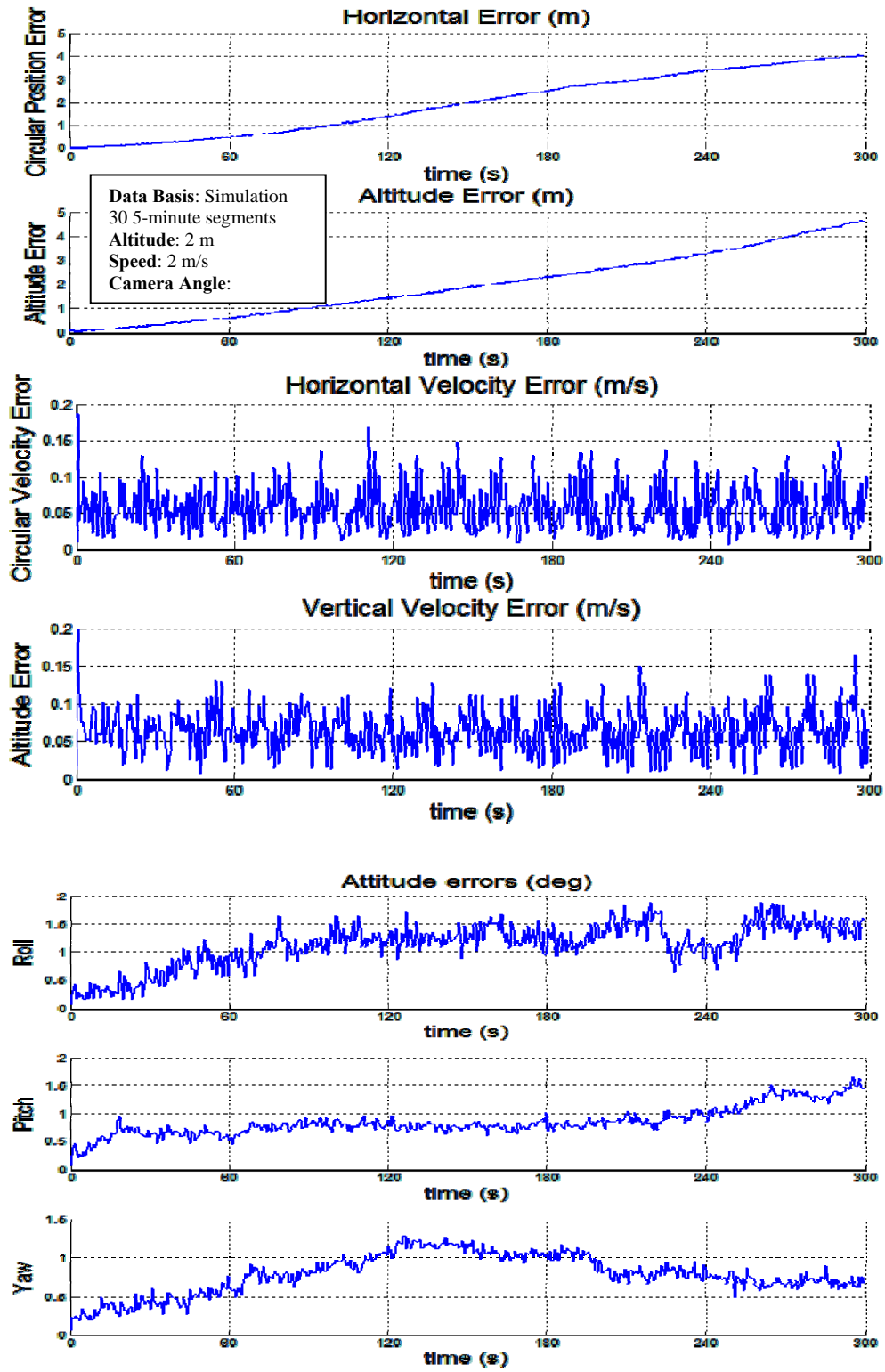
Figure 4.31: Simulated soldier based SLAMR performance.
