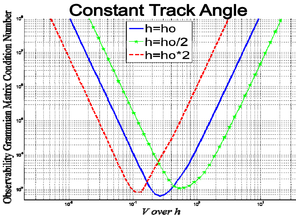
Figure 3.9: Observability gramman matrix condition number as a function of V over h . For a non-dimensionalized case, as altitude ( h ) varies about a nominal height ( h_o ).
