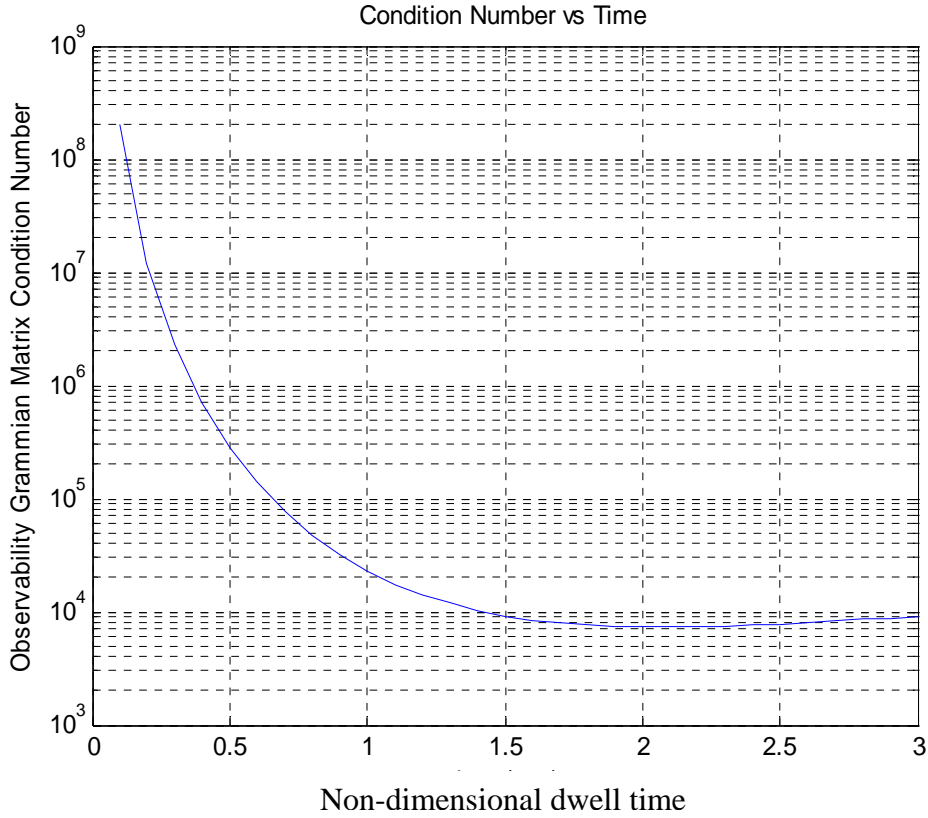
Figure 3.8: Observability gramian matrix condition number vs dwell time in the non-dimensional case study.
