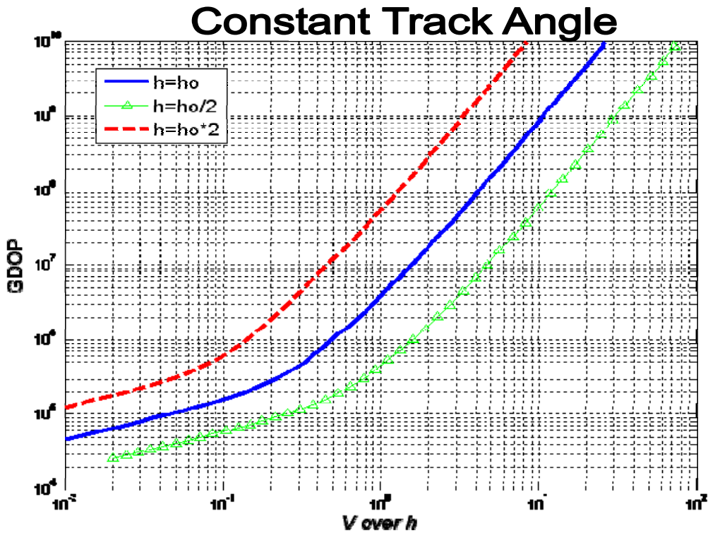
Figure 3.10: Geometric Dilution of Precision as a function of V \text{ over } h . For a non-dimensionalized case, as altitude ( h ) varies about a nominal height ( h_0 ).
