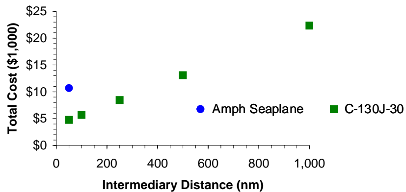
Figure 27: Total cost for maritime patrol/SAR mission
