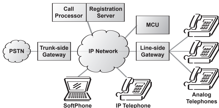
Figure 1: Softphone in a Typical VoIP Configuration
