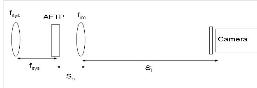
Figure 1. Layout of imaging with magnification experiment.
