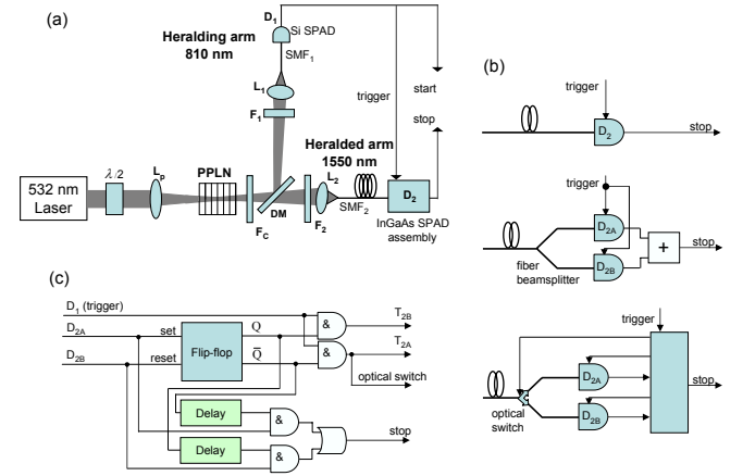
Fig. 3. (a) Setup for testing different arrangements of InGaAs SPAD assemblies; (b) three different InGaAs SPAD assemblies; (c) schematic of electronic logic to actively control InGaAs assemblies and photon routing.
