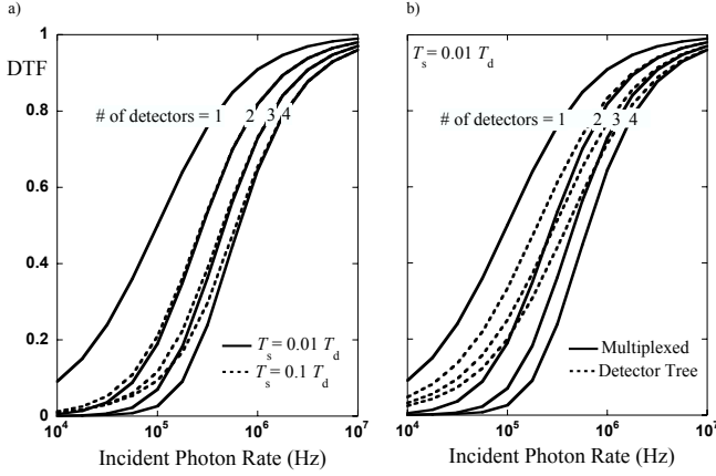
Fig. 2. DTF of multiplexed SPAD systems (a) DTF as a function of incident photon rate for actively switched systems with up to 4 detectors for T_s = 0.01T_d and 0.1T_d ; (b) comparing actively switched assemblies with T_s = 0.01T_d to detector trees shows higher photon rates can be reached at a given DTF.
