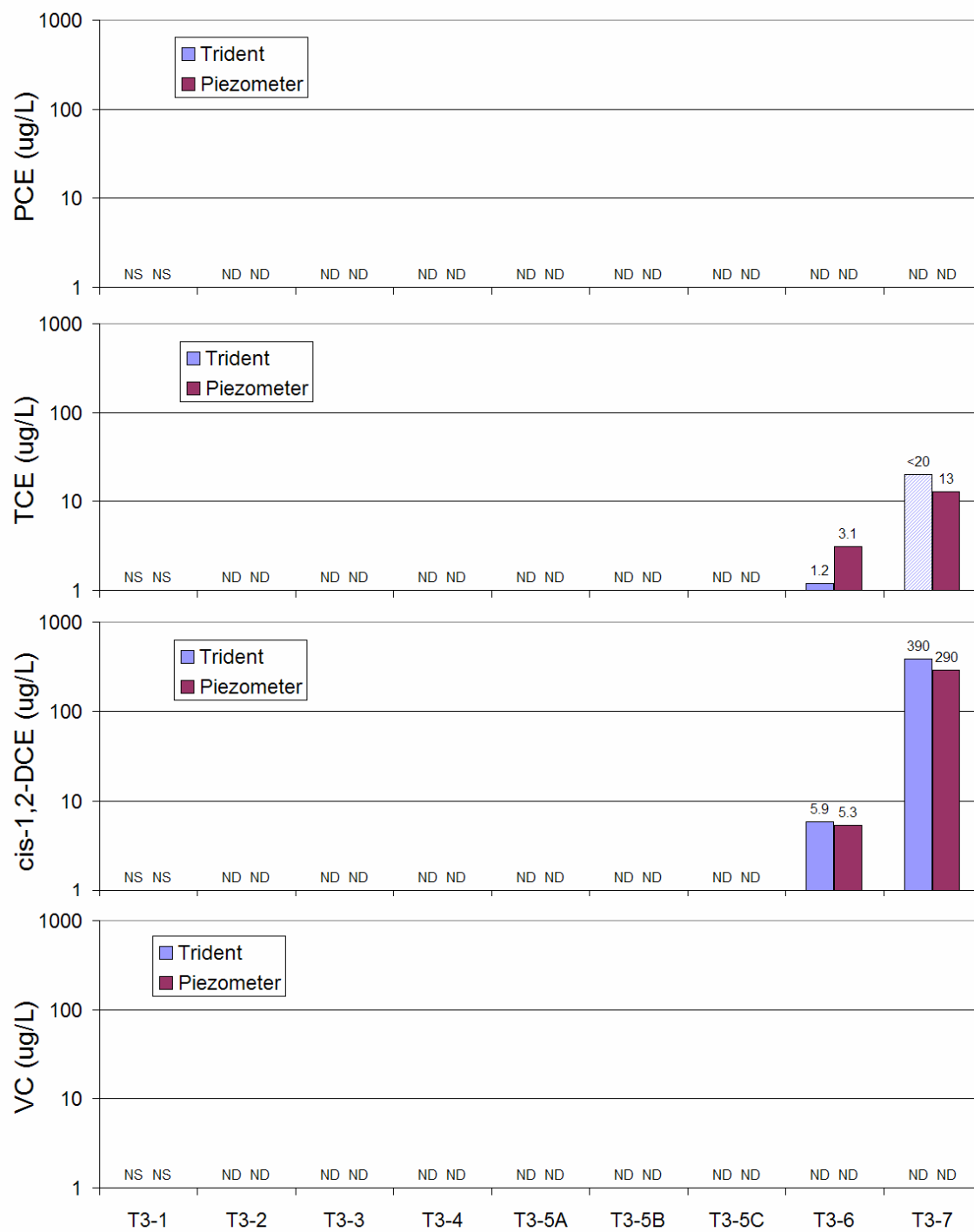
Figure 3-7. Trident probe sub-surface VOC validation along T3.
