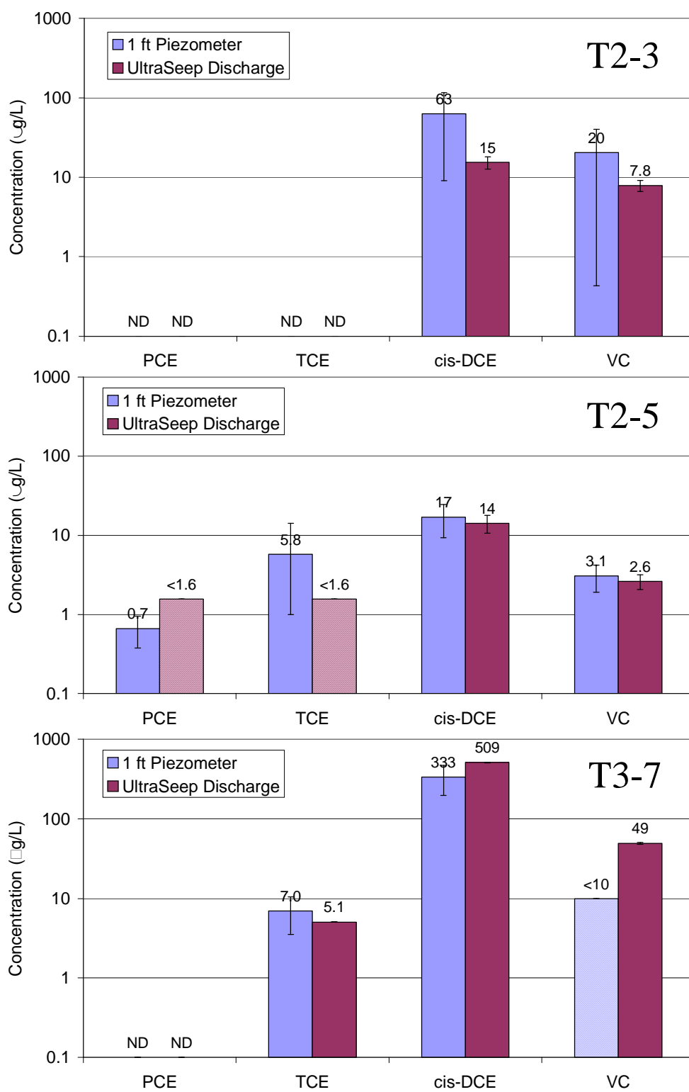
Figure 3-13. UltraSeep VOC validation at each station.
