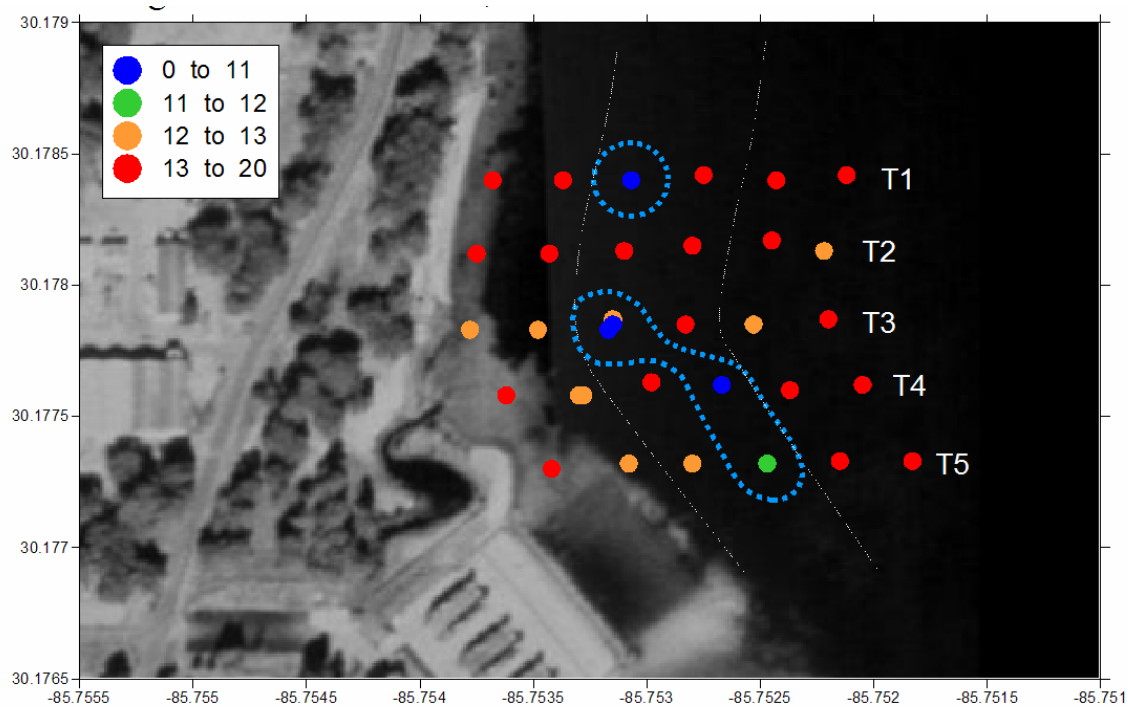
Figure 3-2. Trident probe conductivity map (mS/cm) for the area offshore from AOC 1.
