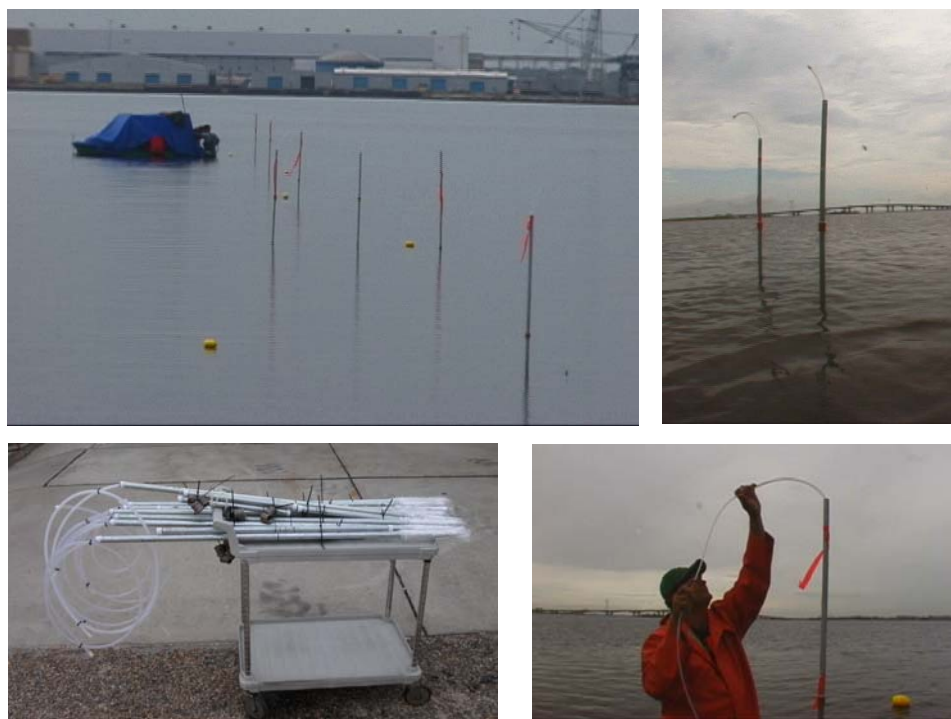
Figure 3-4. Trident probe validation piezometers at AOC 1.
