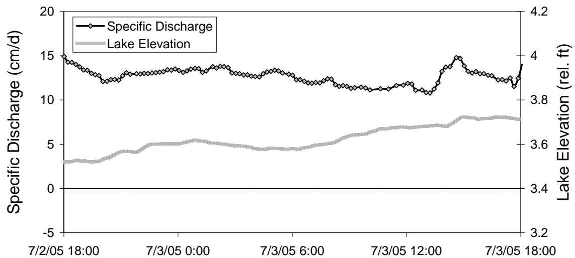
Figure 3-11. Specific discharge and lake level at the T3-7 station.
