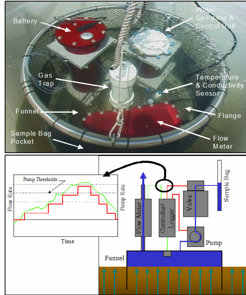
Figure 1-2. The Oceanscience Group commercial UltraSeep system.
