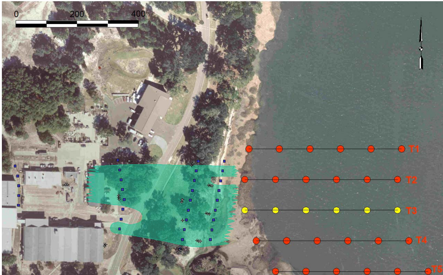
Figure 2-1. Sampling design for the Trident probe survey at NSA Panama City showing historical monitoring wells, DPT locations, approximate location of the 1,1-DCE plume, and proposed offshore transect locations. Red circles indicate stations for Trident probe and surface water sampling and yellow circles indicate stations for Trident probe, surface water, and validation.
