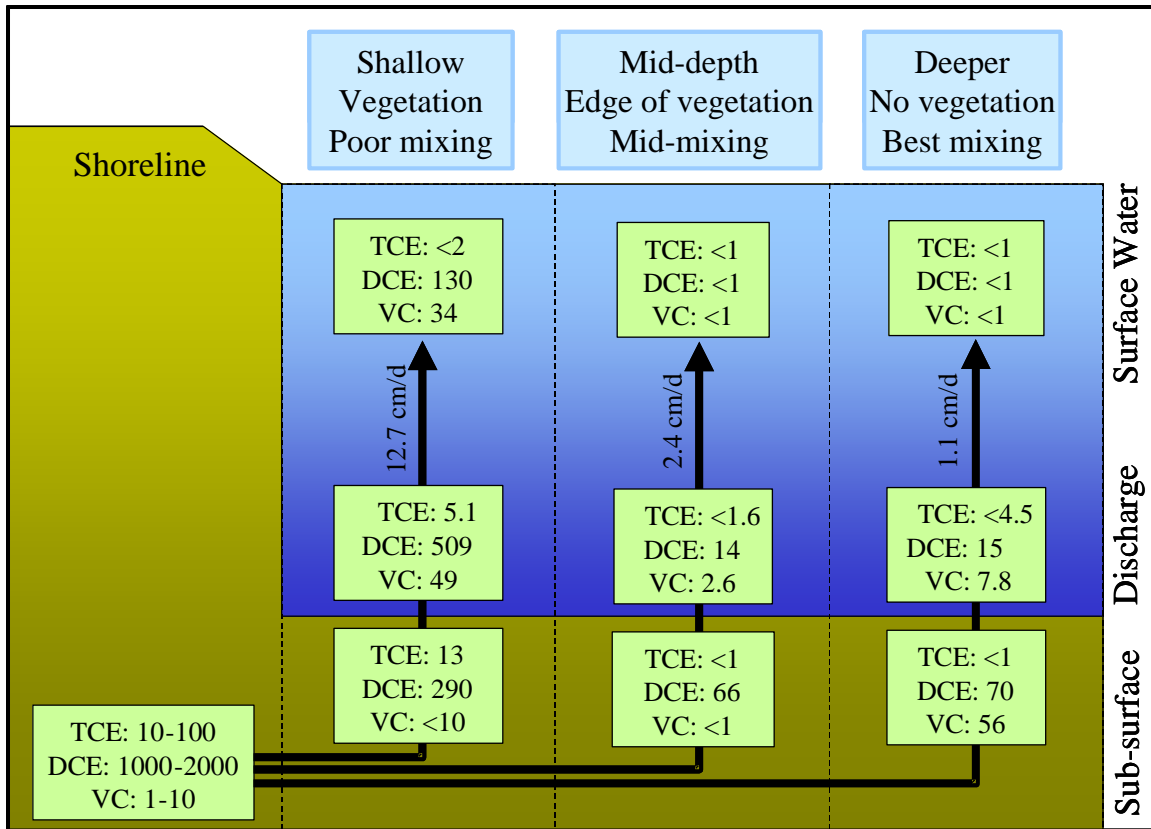
Figure 3-14. Schematic representation of the results from the Trident probe and UltraSeep demonstration at Orlando OU 4.
