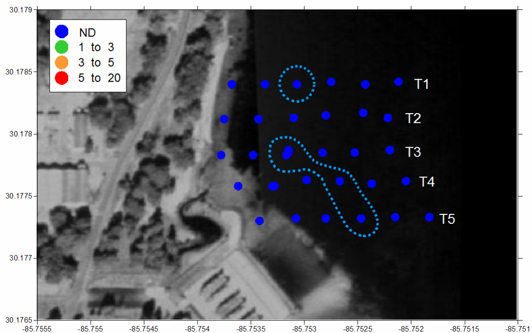
Figure 3-3. Trident probe sub-surface 1,1-DCE map (ug/L) for the area offshore from AOC 1.
