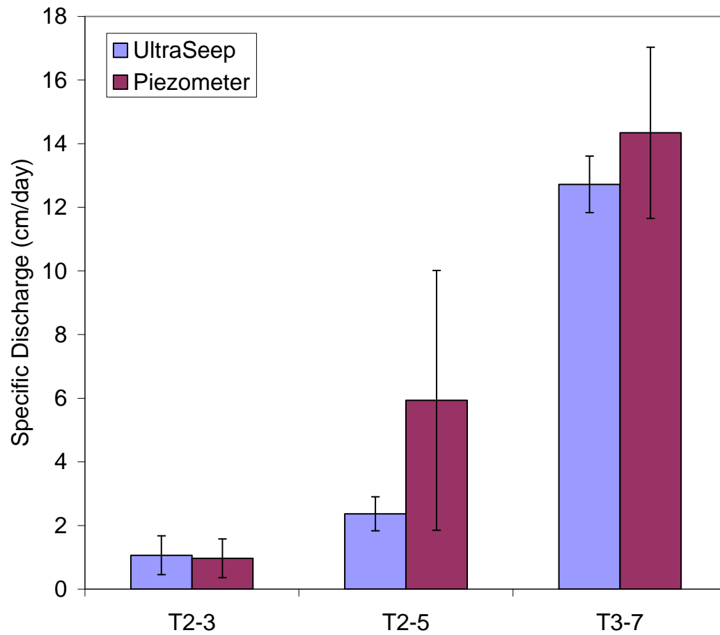
Figure 3-12. UltraSeep flow validation at each station.
