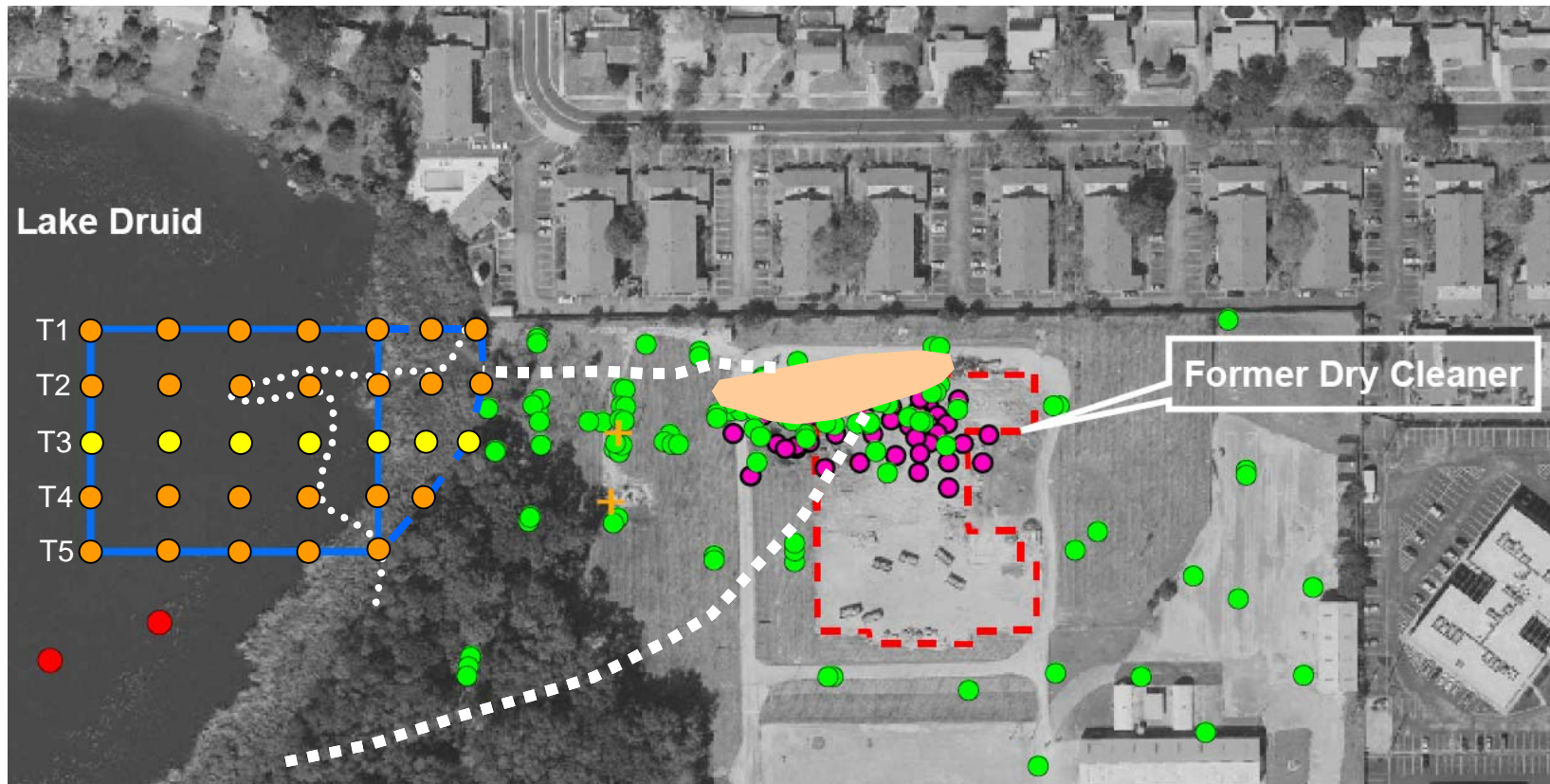
Figure 2-2. Sampling design for the NTC Orlando Lake Druid study area. The orange and yellow dots are the proposed Trident sampling stations. The yellow dots indicate transect T3, where the validation piezometers will be installed.
