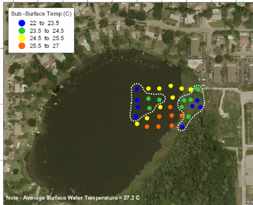
Figure 3-5. Trident probe sub-surface temperature map (° C) for the area offshore of OU 4. Dotted lines indicate groundwater discharge zones based on sub-surface temperature.
