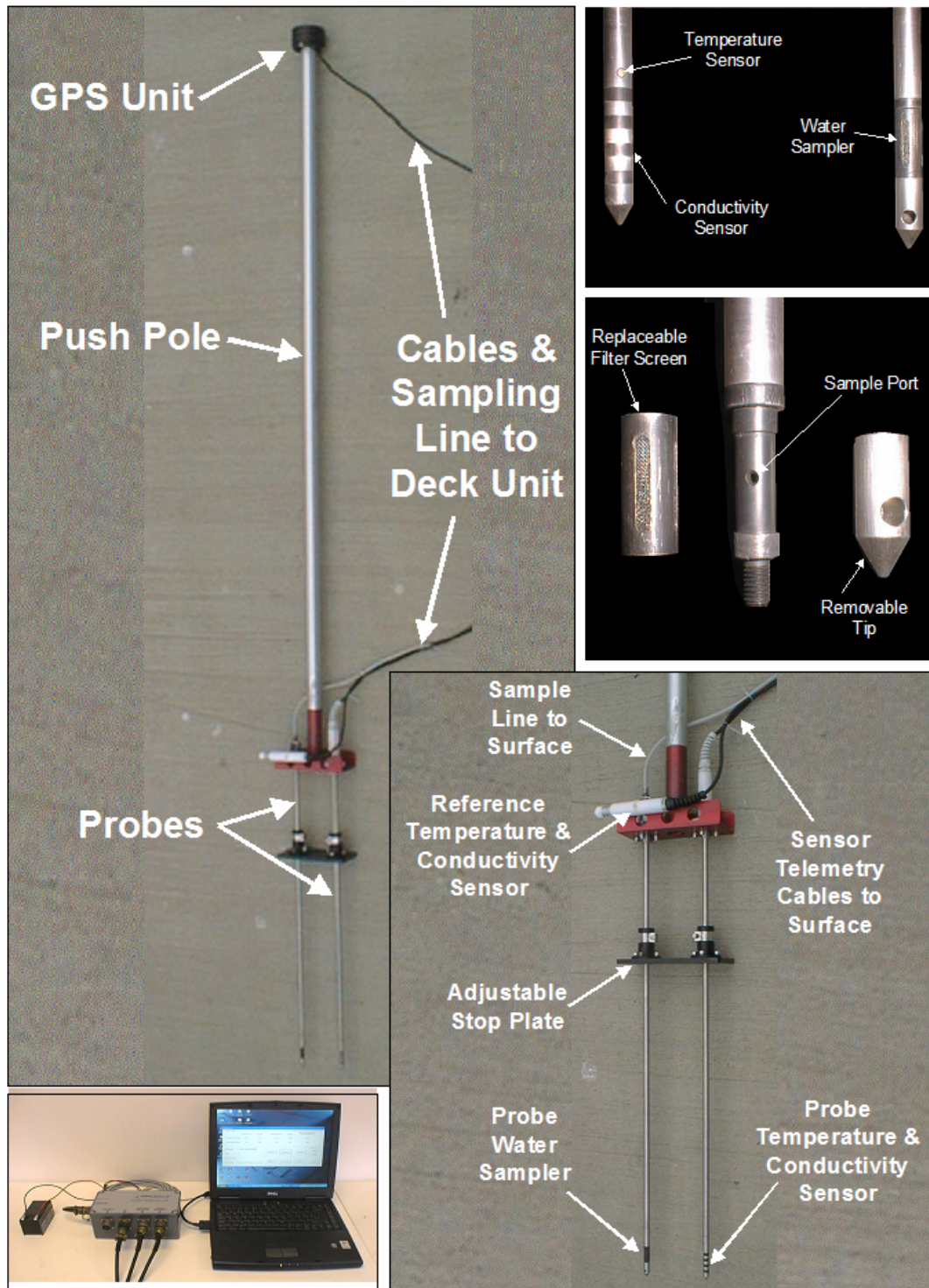
Figure 1-1. Complete Trident probe showing sensor and water sampling probes, push-pole, and Global Positioning System (GPS) unit.
