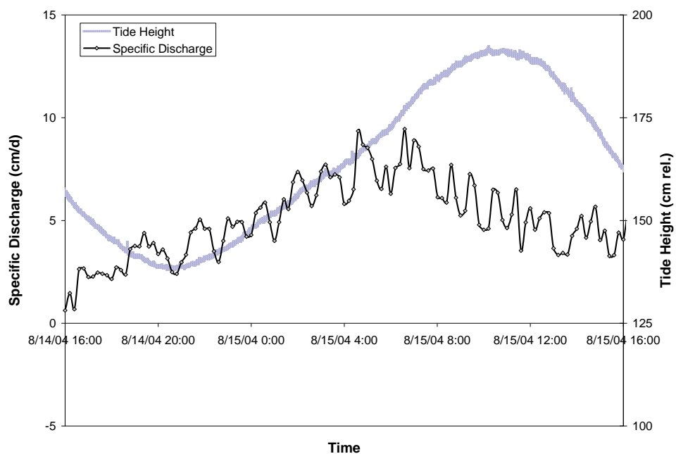
Figure 3-9. Specific discharge and tide height at the T4-4 station.
