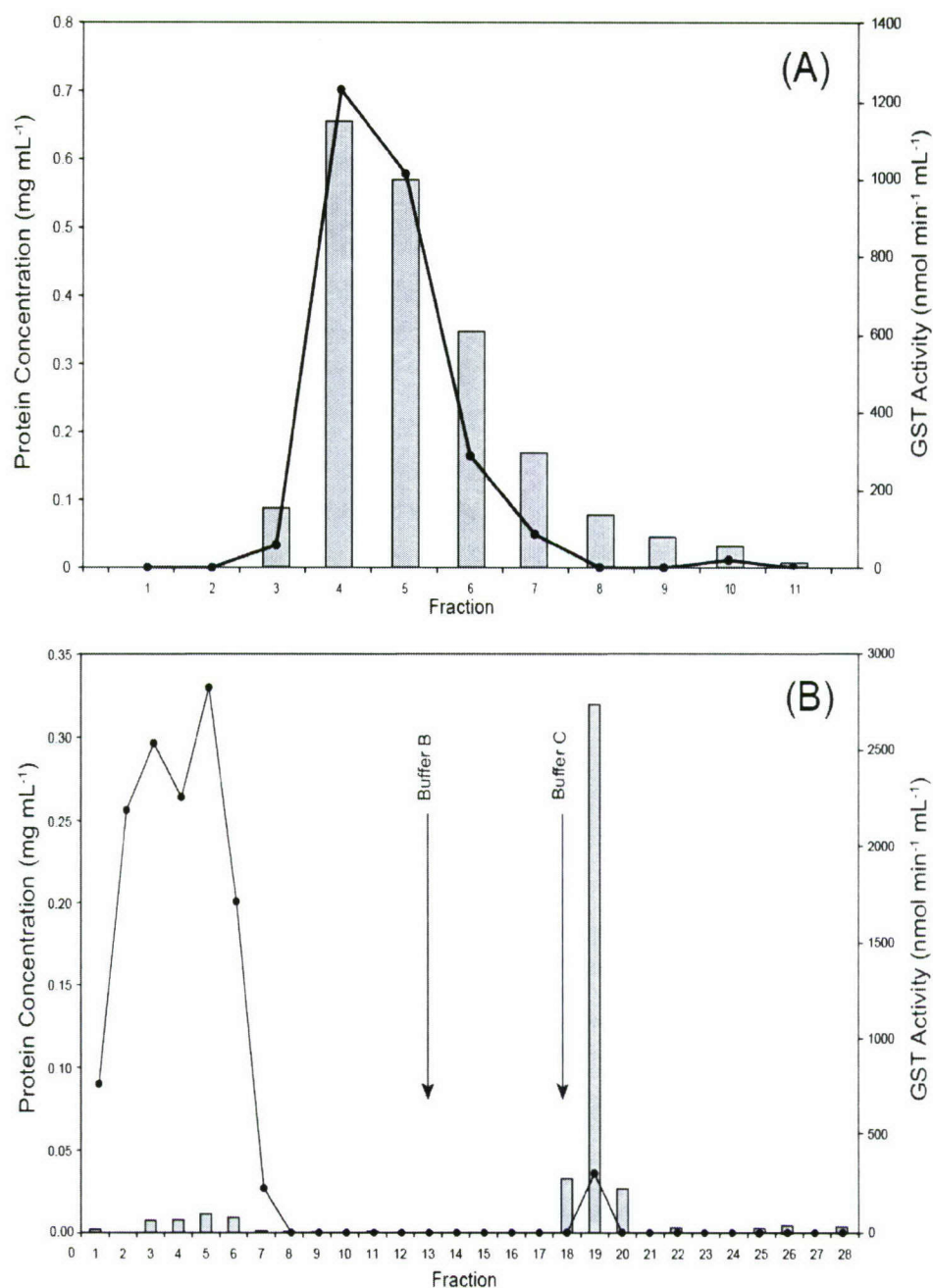
Figure 1. Purification of cytosolic GSTs from C. gibbosum digestive gland. (A) The crude cytosol (2.5 mL) from one individual was applied to a size exclusion PD-10 desalting column (bed volume 8.3 mL, 5 cm height) containing Sephadex G-25 matrix (85 – 260 \mu m) equilibrated in 50 mM Tris buffer, 1mM EDTA, 1mM DTT at pH 6.0 (Buffer A). Fractions were collected in 1.2 mL aliquots by gravity at a flow rate of 1 mL min -1 . Fractions 3 – 7 were pooled for further purification. (B) The pooled fractions (approx. 6 mL) from the size exclusion column were applied to the GSH-agarose (sulfur to epoxide-activated 4% cross-lined beaded agarose) affinity column (bed volume 0.5 mL, 0.8 x 4 cm i.d.) equilibrated in Buffer A. The affinity column was first rinsed with 6 mL of Buffer A and then 7 mL of Buffer B (Buffer A + 0.5 M NaCl) to rinse away non-specific proteins. GSTs were eluted with Buffer C (Buffer B + 50 mM GSH, pH 9.5) in 1 mL aliquots at a flow rate of 0.5 mL min -1 . Fractions 18 -20 were collected and pooled for further separation by HPLC. GST activity (bars) was measured as the increase in absorbance at 340 nm and protein concentration (●) was estimated by absorbance at 595 nm.
