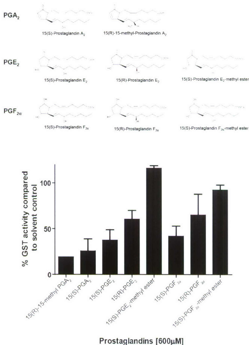
Figure 9. Effect of prostaglandin A, E, and F series on cytosolic C. gibbosum GST activity. Eight commercially available prostaglandin compounds, representing a diversity of prostaglandin series present in gorgonian tissues, were screened for their ability to inhibit GST activity at 600 \mu M. Bars represent the mean ( \pm SE) percent GST activity remaining after prostaglandin exposure compared to solvent controls. The reaction mixture consisted of 2 \mu g of cytosolic GST protein in 0.1 M potassium phosphate buffer, pH 7.5, containing 1 mM GSH, 1 mM CDNB at 25°C with 5% (v/v) DMSO. Digestive gland cytosolic preparations from two snails were used as the enzyme source with specific activities of 5.8 and 5.1 \mu mol min -1 mg protein -1 , respectively.
