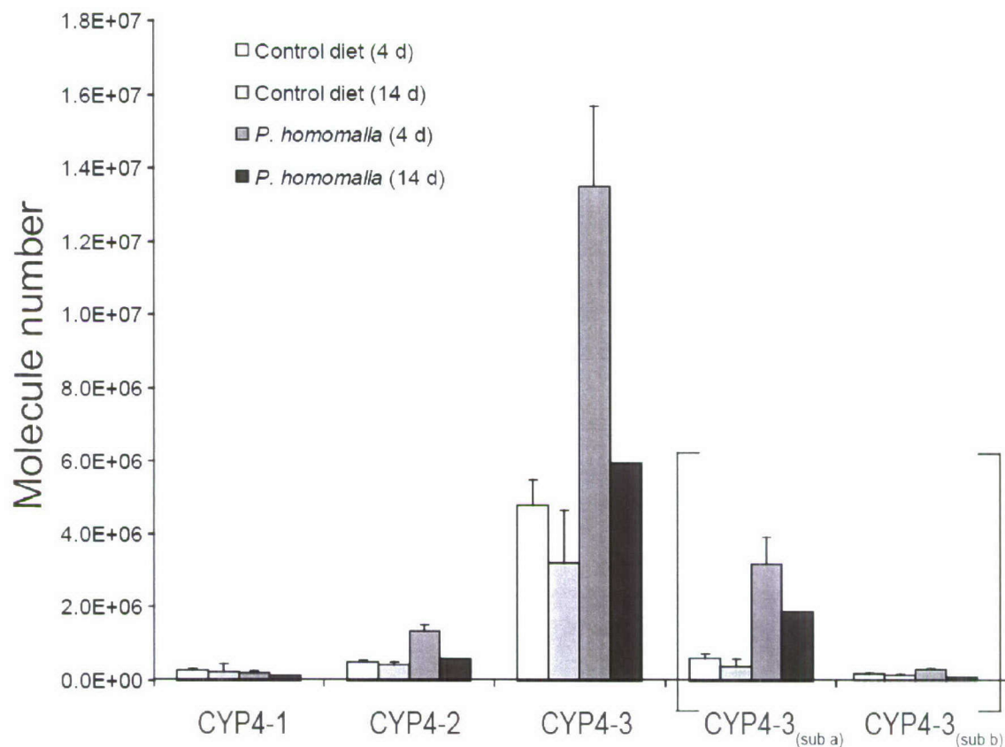
Figure 19. Comparison of CYP4 gene expression in snails feeding on control or P. homomalla diet for 4 d or greater. Bars represent the mean CYP4 gene expression ( \pm SE) of snails feeding on control diet ( n = 27 snails; e.g. alginic acid + squid powder) or P. homomalla ( n = 9 snails) for 4d. Results shown here only include snails from four reefs (Big Point, North Normans, Rainbow Gardens, and Sugar Blue Holes). Run in parallel to the four day feeding assays was a series of long term feeding assays used to examine the induction of CYP4 in C. gibbosum . Adult C. gibbosum collected from North Normans were allowed to feed on control ( n = 2 ) or P. homomalla ( n = 1 ) for 14 d and mean CYP4 gene expression ( \pm SE) is shown for each 14 d diet group. Real-time quantitative PCR was performed and the number of molecules per 0.2 \mu g of polyA + RNA was calculated from the standard curve and normalized by a \beta -actin correction factor. Bars in the [ ] indicate molecule numbers for a subset of genes within group CYP4-3.
