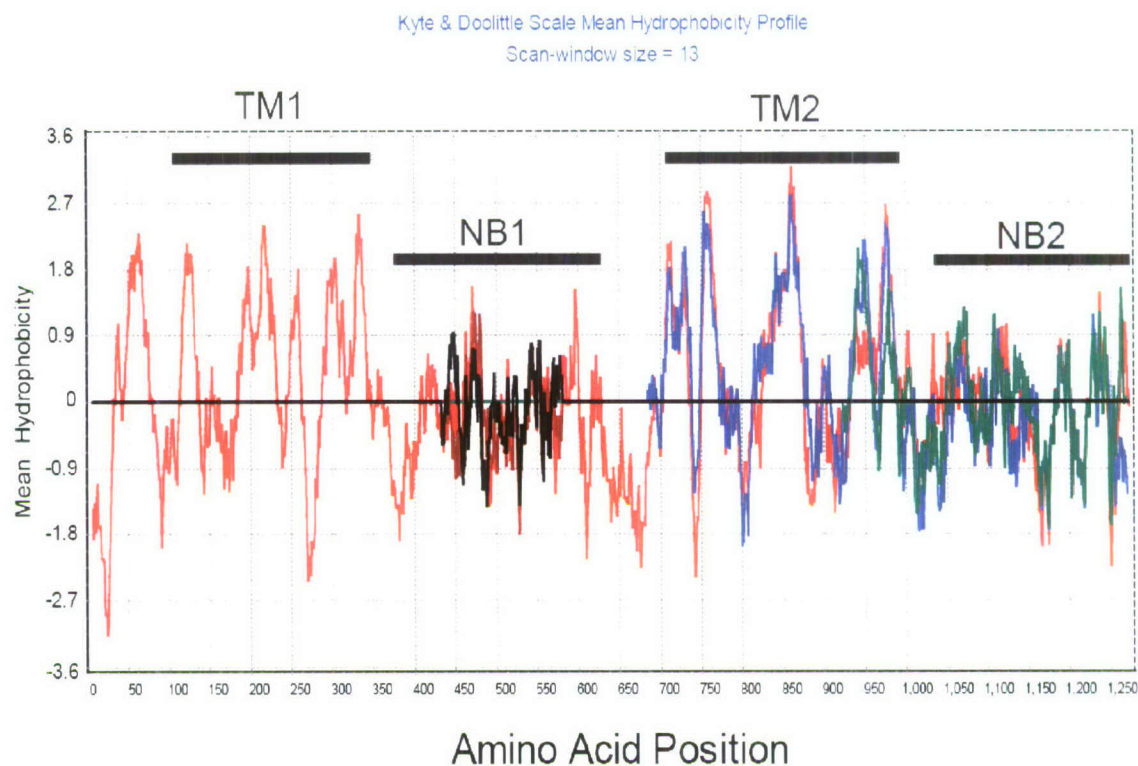
Figure 12. Comparison of molluscan and mouse Pgp hydropathy profiles. Deduced amino acid sequences of Cyphoma and Tritonia P-glycoproteins were aligned to mouse ABCB1a using ClustalX. The mouse ABCB1a plot is indicated by the red line and is overlaid by Cyphoma Pgp-1 (blue line), Cyphoma Pgp-2 (green line), Tritonia Pgp-1 (maroon line), and Tritonia Pgp-2 (black line). Black bars above the plots indicate positions of the two transmembrane regions (TM1, TM2) and nucleotide binding domains (NB1, NB2) in ABCB proteins. Values above and below the horizontal line indicate hydrophobic and hydrophilic regions, respectively. Hydrophobicity plots were generated using the Kyte-Doolittle algorithm (1982) with a window of 13 residues by BioEdit v7.0.5.2. GenBank sequences in the alignment include: mouse ABCB1a ( M. musculus , NP_035206), C. gibbosum Pgp-1 (EU487190), C. gibbosum Pgp-2 (EU487191), T. hamnerorum Pgp-1 (EU487196), T. hamnerorum Pgp-2 (EU487197).
