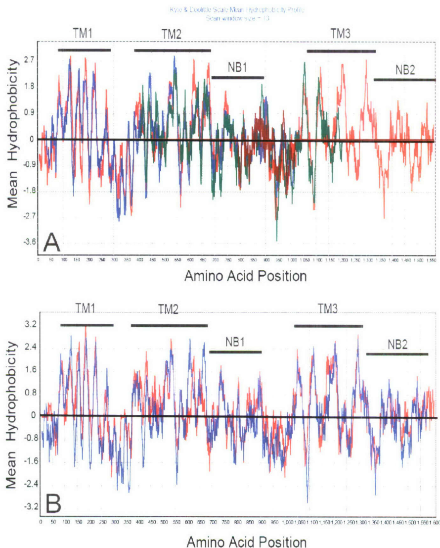
Figure 11. Comparison of molluscan and human MRP hydropathy profiles. (A) Deduced amino acid sequences from Cyphoma and Tritonia MRP profiles were aligned using ClustalX. Tritonia MRP-1 plot is indicated by the red line and the Cyphoma MRP-1 (blue line), Tritonia MRP-2 (green line) and Cyphoma MRP-2 (maroon line) are layered on top. (B) Deduced amino acid sequence from Tritonia MRP-1 (blue line) was aligned with human ABCC3 (red line) using ClustalX. Black bars above the plots indicate positions of the three transmembrane regions (TM1, TM2, TM3) and nucleotide binding domains (NB1, NB2) in ABCC proteins. Values above and below the horizontal line indicate hydrophobic and hydrophilic regions, respectively. Hydropobicity plots were generated using the Kyte-Doolittle algorithm (1982) with a window of 13 residues by BioEdit v7.0.5.2. GenBank sequences in the alignment include: human ABCC3 (NP_003777.2), C. gibbosum MRP-1 (EU487192), C. gibbosum MRP-2 (EU487193), T. hamnerorum MRP-1 (EU487194), T. hamnerorum MRP-2 (EU487195).
