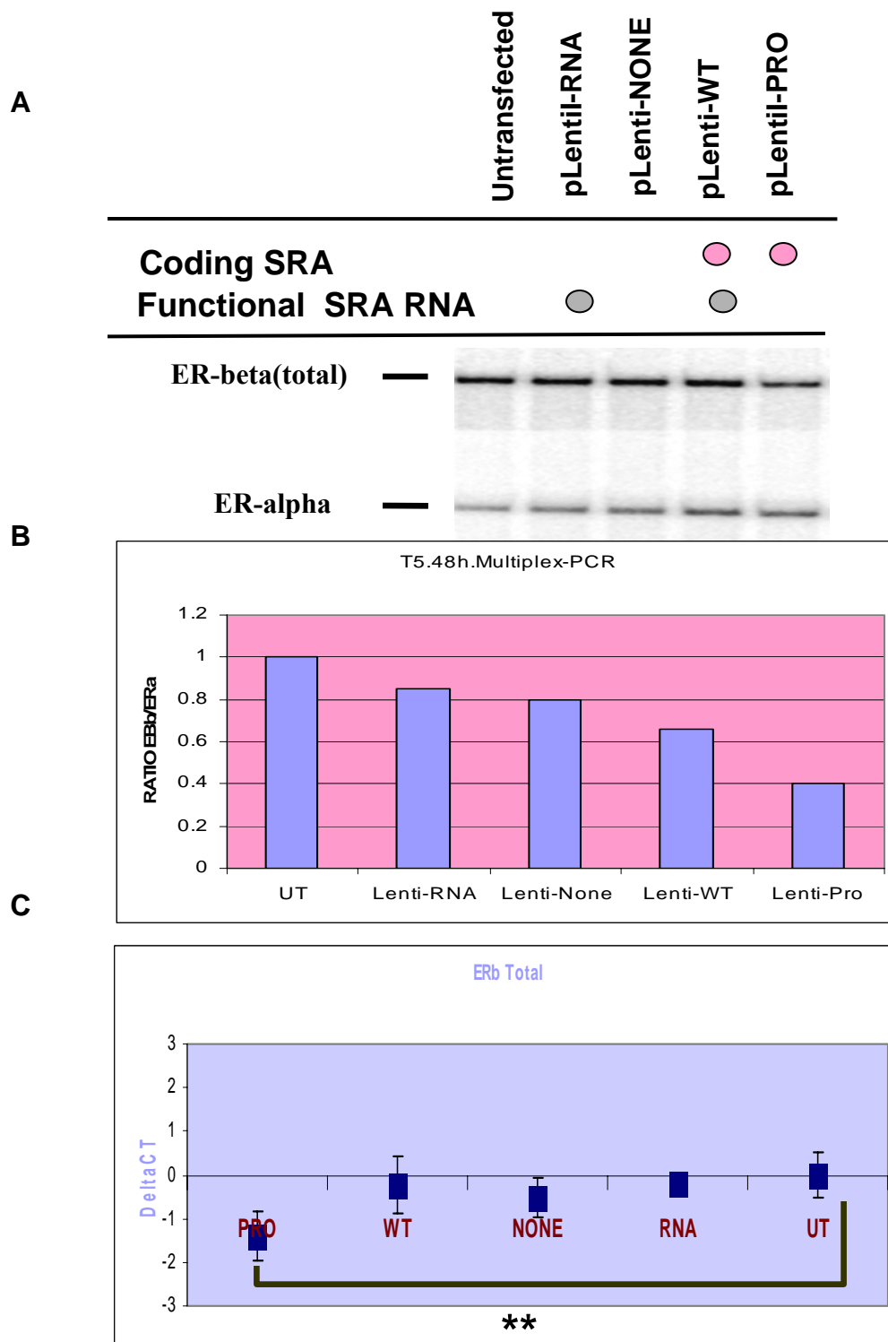
Figure 4: SRAP down regulates the ERbeta expression in mRNA level.
