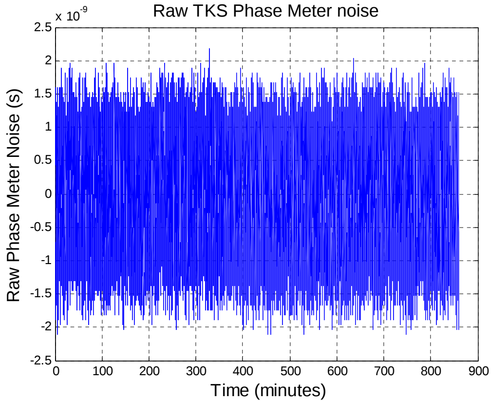
Figure 4. Raw TKS phase meter noise.
