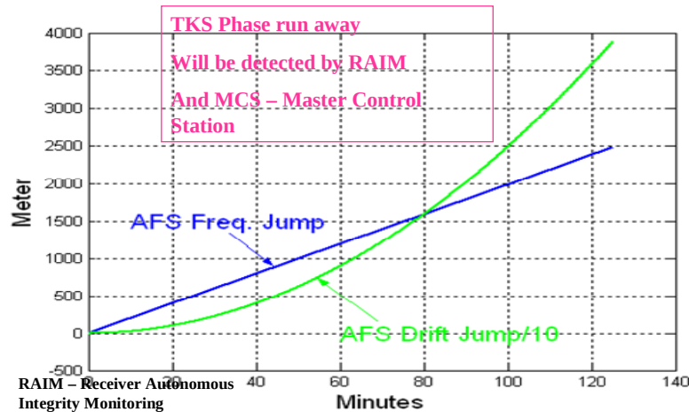
Figure 10. TKS phase runaway due to a RAFS frequency jump and frequency drift jump.
