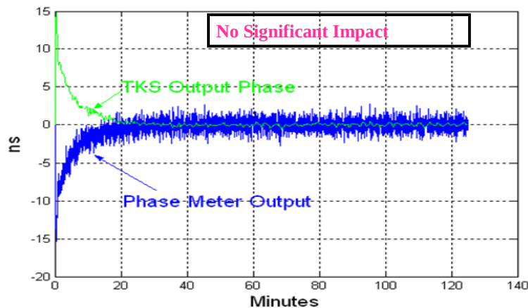
Figure 8. TKS phase transients due to a VCXO frequency jump.
