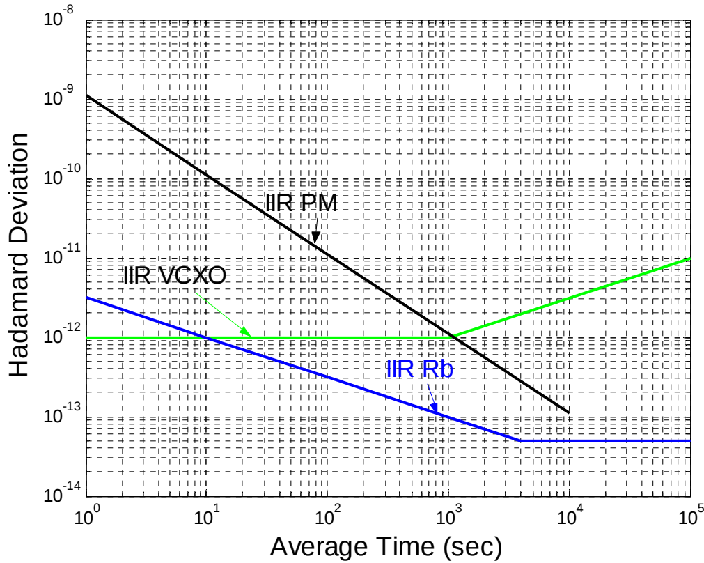
Figure 2. Hadamard deviation of the TKS components.
