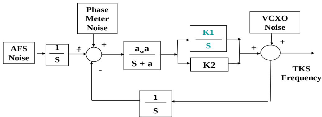
Figure 3 Simplified TKS Error Model in S Domain
