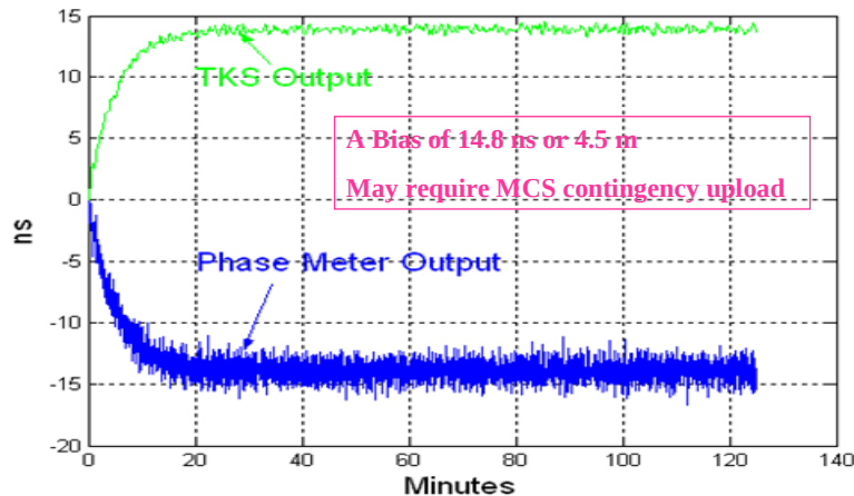
Figure 9. TKS phase transients due to a VCXO frequency drift jump.
