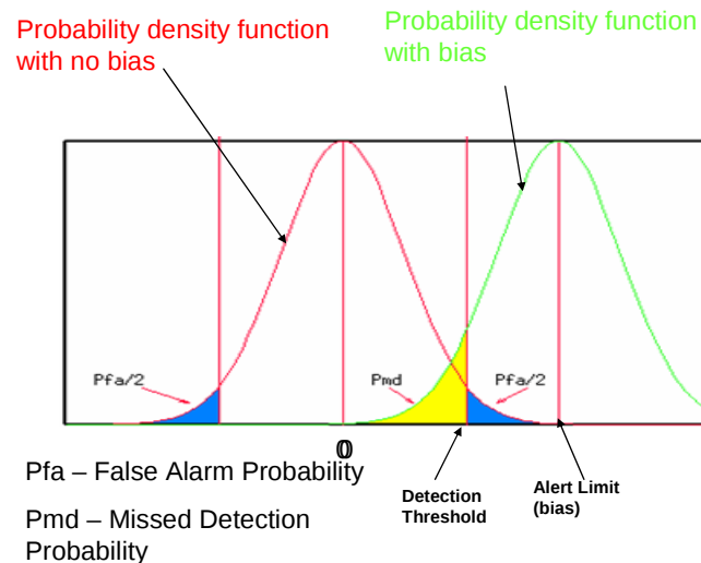
Figure 7. Integrity monitoring parameters.
