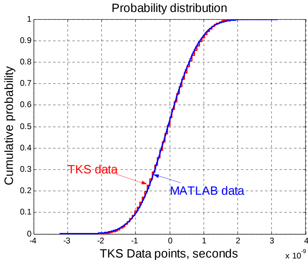
Figure 5. Cumulative probability functions.
