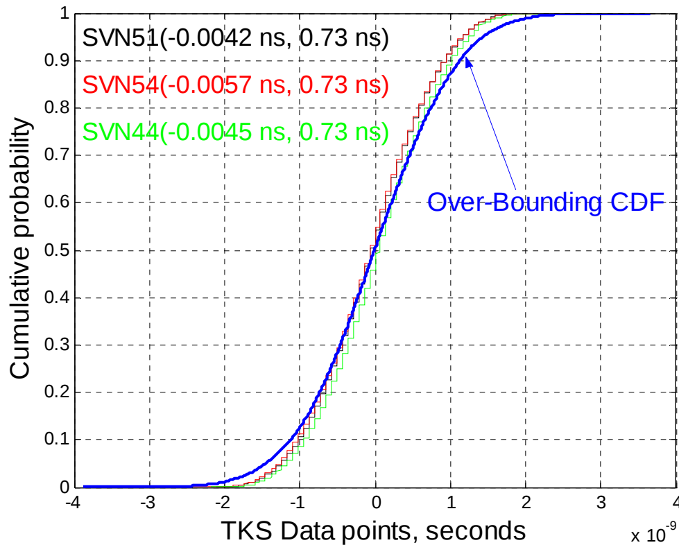
Figure 6. Over-bounding cumulative probability distribution function.
