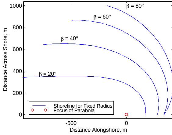
Fig. 5. Parabolic shape for selected values of angle \beta ( R_0 = 1,000 m).
