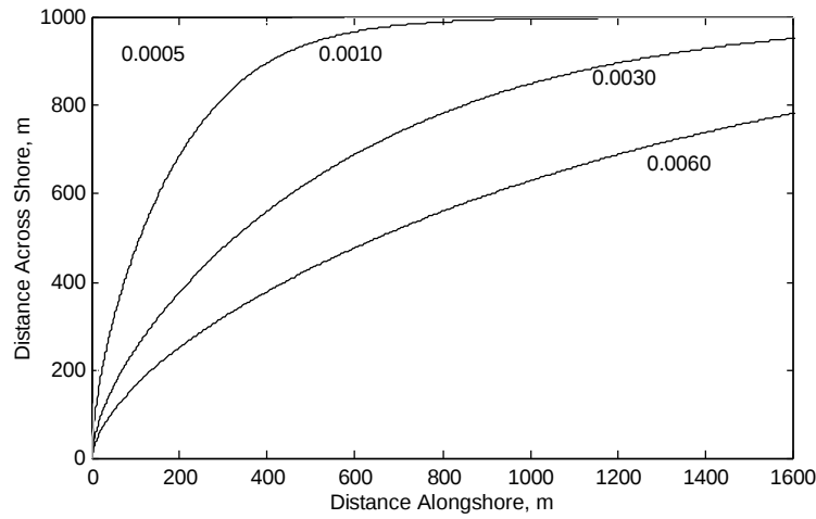
Fig. 8. Dependence of hyperbolic-tangent shape on b ( a = 1,000 m; m = 0.6 ).
