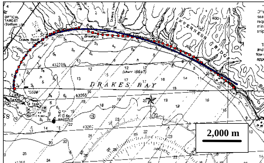
Fig. 11. Hyperbolic-tangent fit to Drakes Bay, California.
