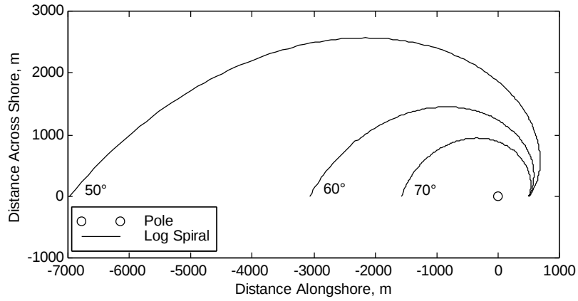
Fig. 2. Variation of logarithmic-spiral shape with \alpha ( R_0 = 500 m).
