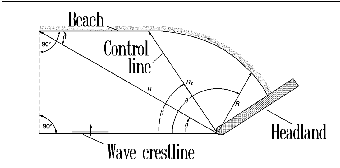
Fig. 4. Definition sketch of the parabolic shape.
