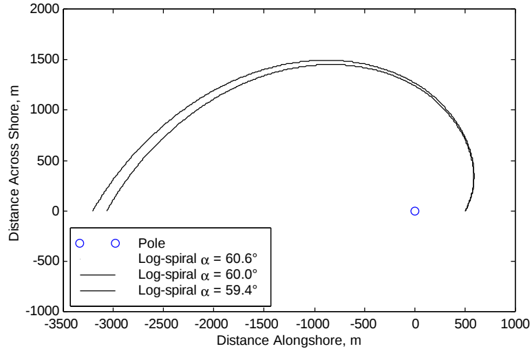
Fig. 3. Sensitivity of log-spiral shape to small variations of the parameter \alpha ( R_0 = 500 m).
