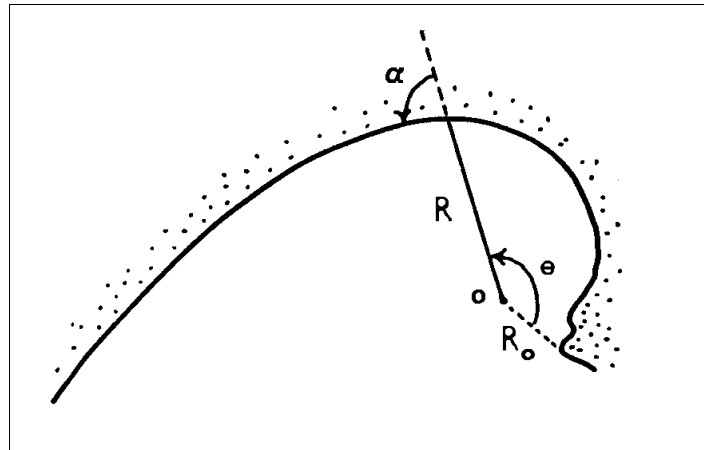
Fig. 1. Definition sketch of the logarithmic spiral shape.
