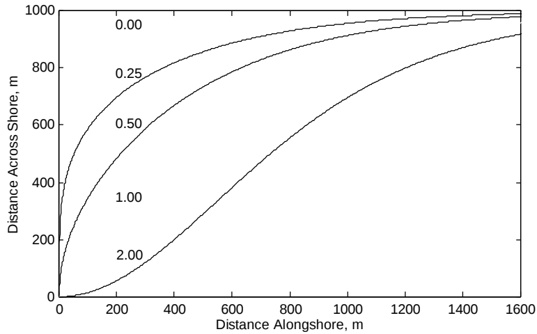
Fig. 9. Dependence of hyperbolic-tangent shape on m ( a = 1,000 m; b = 0.0012 m -1 ).
