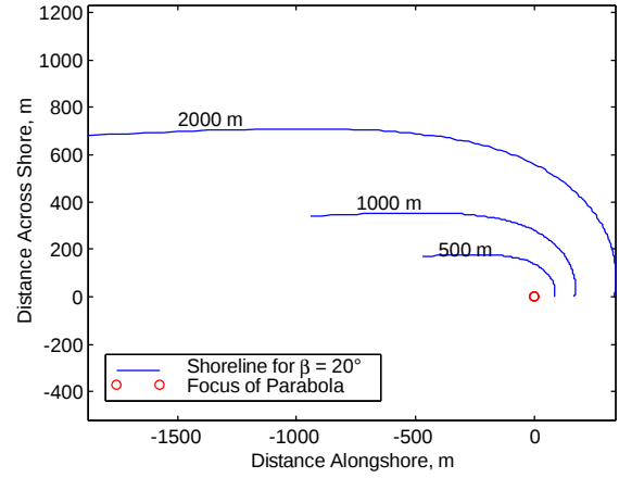
Fig. 6. Parabolic shape for selected values of R_0 ( \beta = 20^\circ ).
