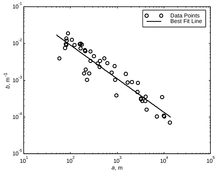
Fig. 10. Plot of a versus b values for hyperbolic-tangent shape and best-fit line.
