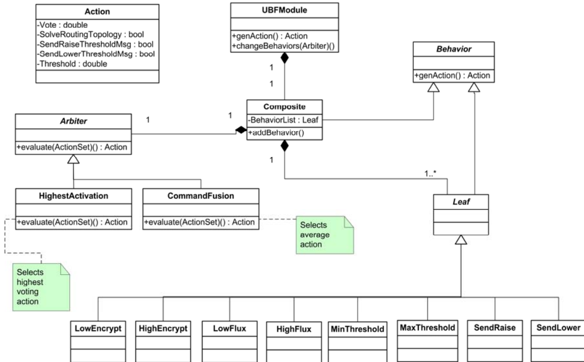
Figure 3-8: UML Diagram for the UBF Module. The UBF's composite behavior consists of an Arbiter and several Leaf Behaviors. The Leaf Behaviors generate candidate actions that the arbiter combines into a single action. The action is returned to the Agent.
