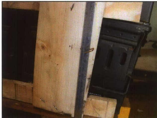
Photo 11. Disengaged Staple During Incline-Impact Testing of Test Unit #1.
