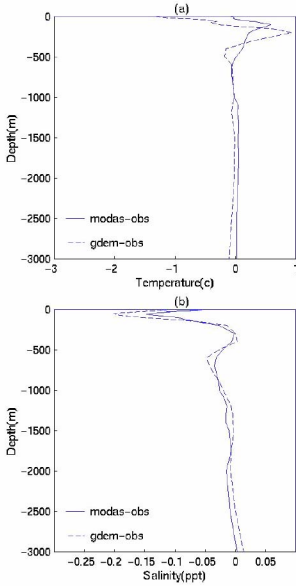
Fig. 9. The BIAS between the MODAS and SCSMEX data (solid) and between the GDEM and SCSMEX data (dotted): (a) temperature ( ^{\circ}\text{C} ), and (b) salinity (ppt).
