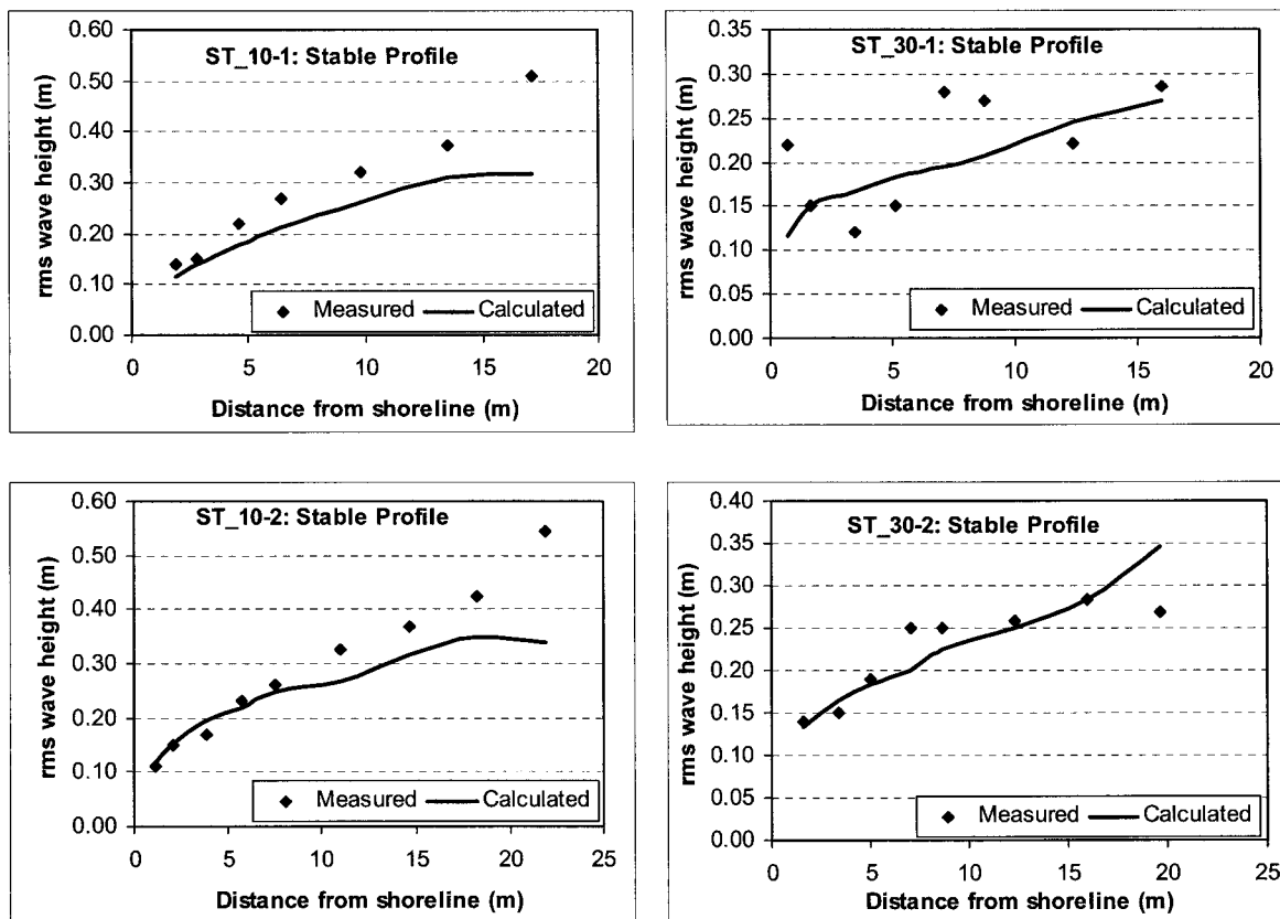
Figure 8. Measured and predicted (Eq. 6) wave heights across the surf zone, irregular wave cases.
