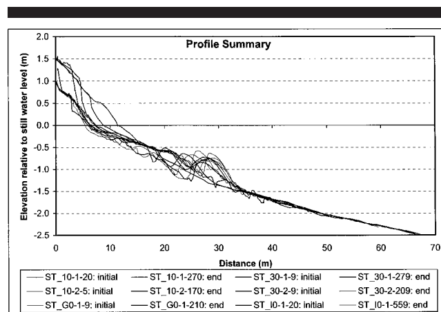
Figure 1. All beach profiles examined in this study; note that the profile changed little seaward of the bar.
