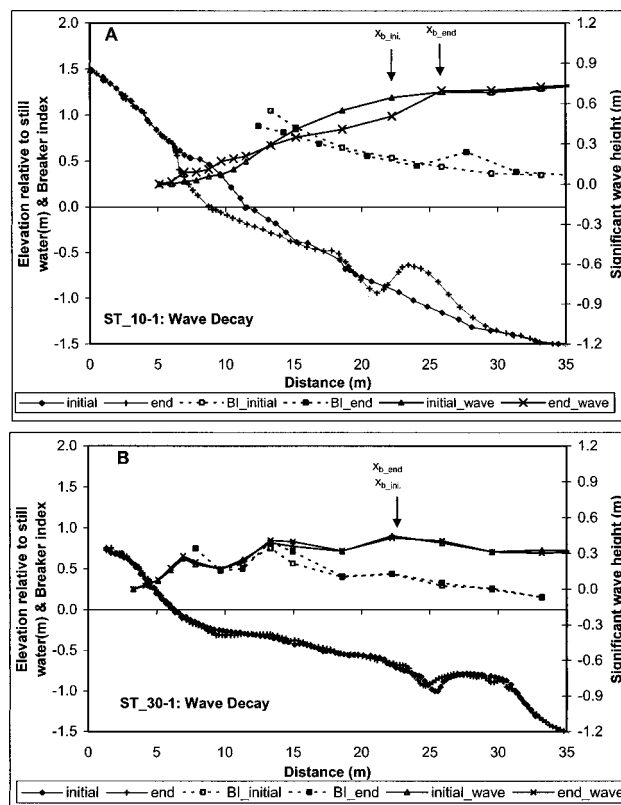
Figure 5. Cross-shore distributions of wave-height decay and breaker index over the initial and end beach profile for ST_10-1 and ST_30-1.
