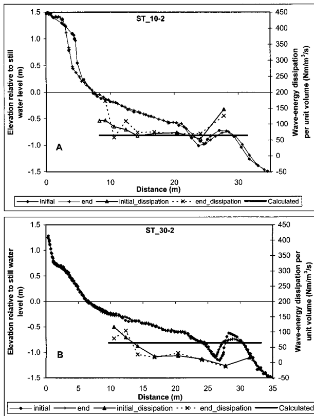
Figure 11. Wave-energy dissipation rate per unit volume over the initial and end beach profiles, and the computed equilibrium dissipation rate for ST-10-2 and ST-30-2.
