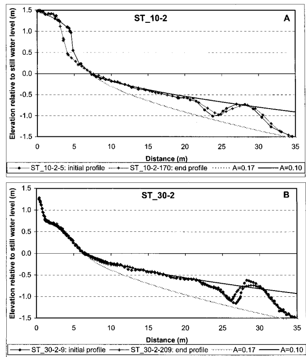
Figure 3. Initial and end beach profiles for ST.10-2 and ST.30-2, and the power-function profiles.
