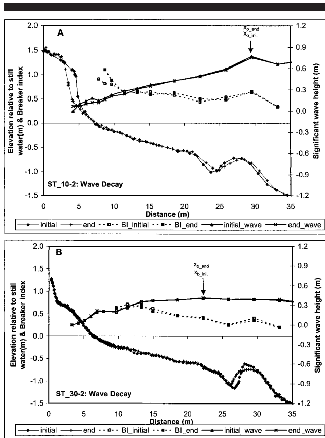
Figure 6. Cross-shore distributions of wave-height decay and breaker index over the initial and end beach profile for ST_10-2 and ST_30-2.
