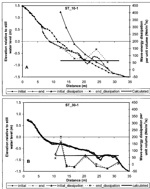
Figure 10. Wave-energy dissipation rate per unit volume over the initial and end beach profiles, and the computed equilibrium dissipation rate for ST.10-1 and ST.30-1.
