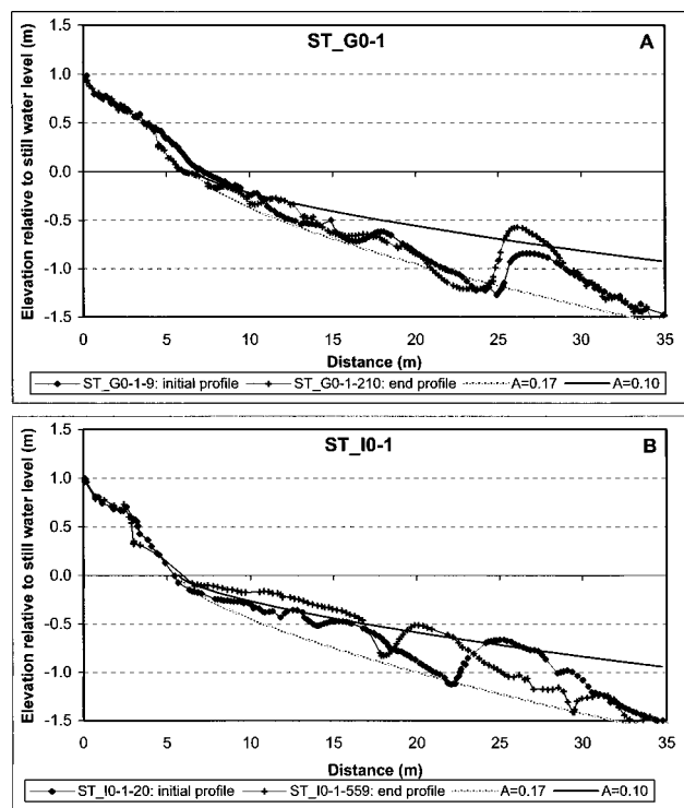
Figure 4. Initial and end beach profiles for ST_G0-1 and ST_I0-1, and the power-function profiles.
