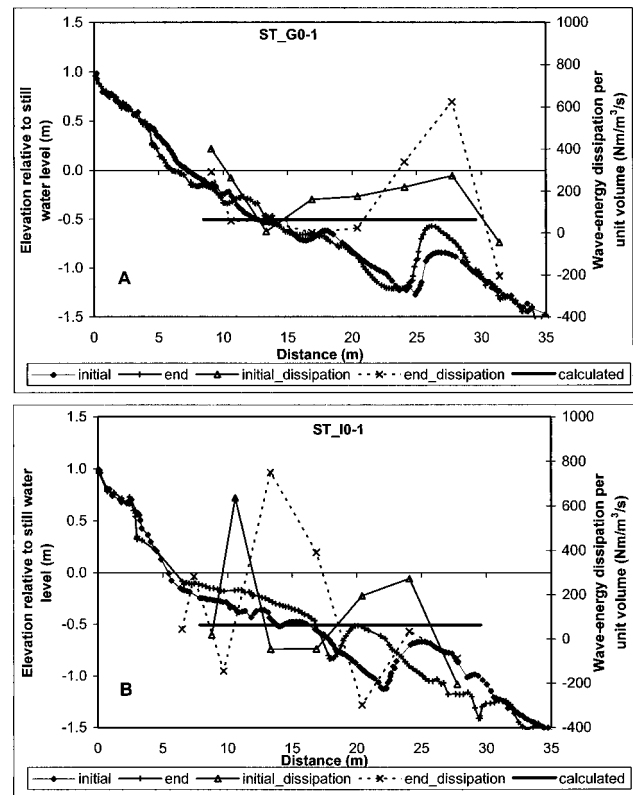
Figure 12. Wave-energy dissipation rate per unit volume over the initial and end beach profiles, and the computed equilibrium dissipation rate for ST-G0-1 and ST-I0-1.
