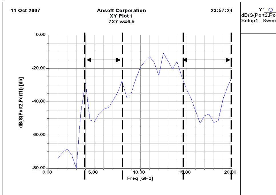
Figure 54. Patch width optimization w=6.5 mm (band gap occurs between 4-8 GHz and 15-20 GHz)
