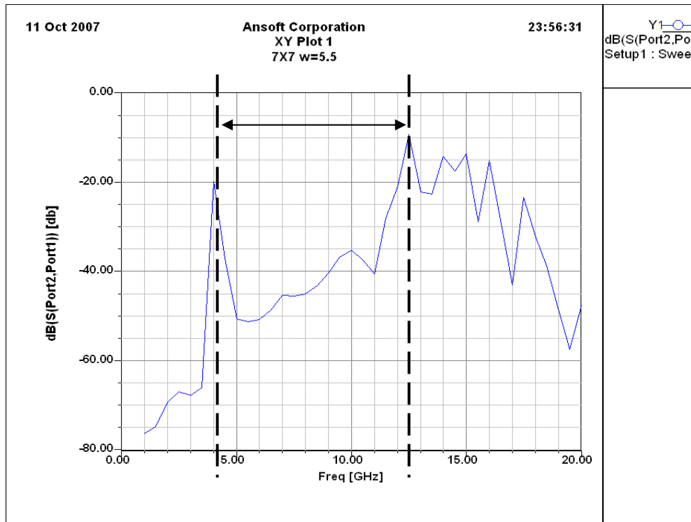
Figure 53. Patch width optimization w=5.5 mm (band gap occurs between 4-12.5 GHz)
