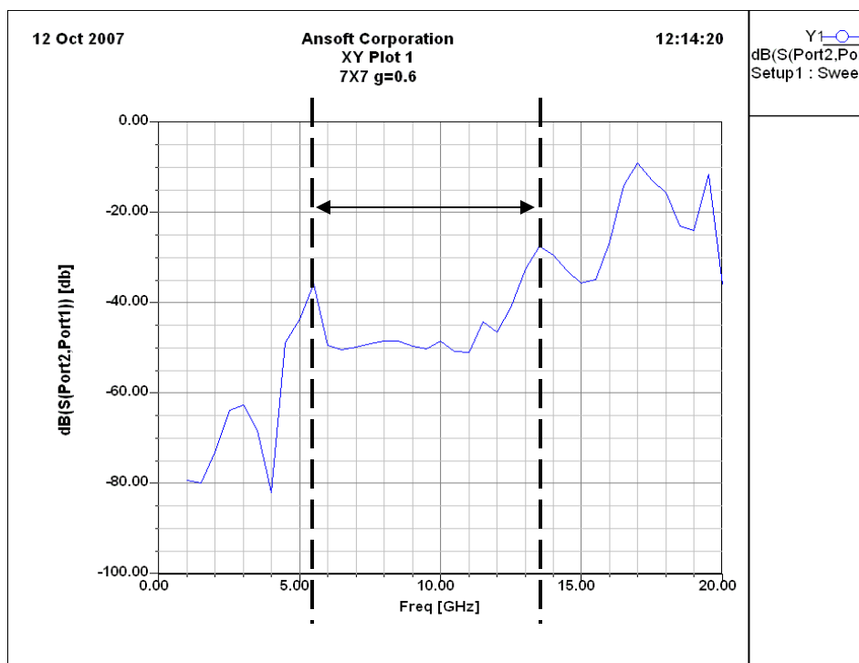
Figure 57. Gap width optimization g=0.6\text{mm} (band gap = 5.5-13.5 GHz)
