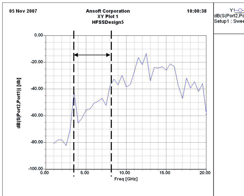
Figure 93. S_{21} Hexagon patch w=6.5\text{mm} (band gap= 3.5-8 GHz)
