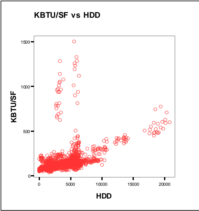
Figure 4-1. Scatter plot of KBTU/SF vs. HDD
