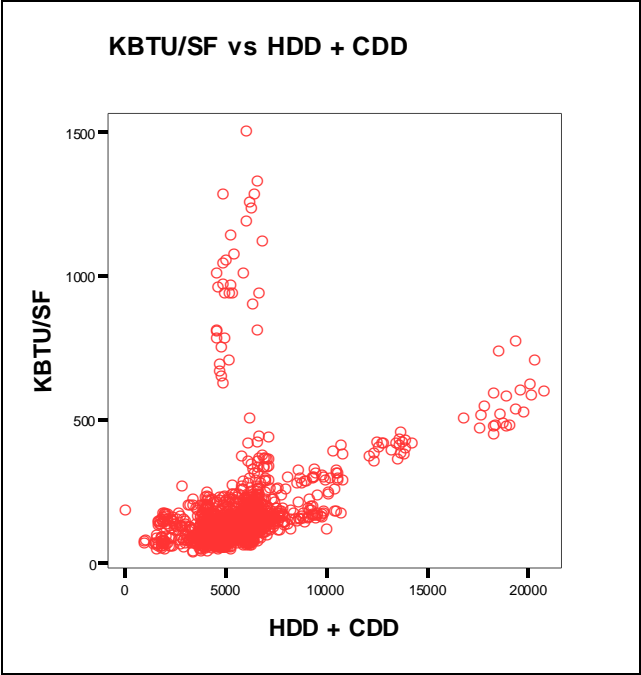
Figure 4-3. Scatter plot of KBTU/SF vs. HDD + CDD
