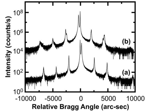
FIG. 4. XRD spectra of InAs/GaSb superlattices, [(\text{InAs})_{13}/(\text{GaSb})_{13}]_{140} , grown at 390^\circ\text{C} using (a) \text{As}_2 and (b) \text{As}_4 . The spectra are plotted relative to the Bragg angle for bulk GaSb. In (a) the epilayer peak (the peak just off zero) is at a larger Bragg angle than the GaSb substrate peak, indicating that the average lattice constant of the superlattice is smaller than that of GaSb. Conversely, in (b), the position of the epilayer peak indicates a lattice constant smaller than the substrate.
