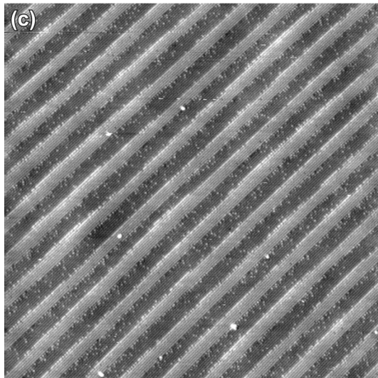
FIG. 3. InAs/GaSb superlattices grown at 390^\circ\text{C} using (a) \text{As}_2 and (b), (c) \text{As}_4 with an \text{As}_4 :In flux ratio of 2.0:1. The images in (a) and (b) are 55\text{ nm}\times 55\text{ nm} , and in (c) 110\text{ nm}\times 110\text{ nm} .
