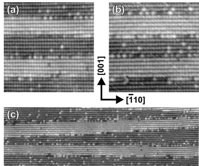
FIG. 2. InAs/GaSb heterostructures grown at 425 °C using As 4 . The GaSb layers were exposed to an As 4 flux at the InAs-on-GaSb interfaces for (a) 5 s and (b) 30 s (images 15 nm×15 nm). There is little evidence of GaAs interfacial bonds at the InAs-on-GaSb interfaces. (c) A larger-scale image, 18 nm×60 nm, of the heterostructure shown in (b).
