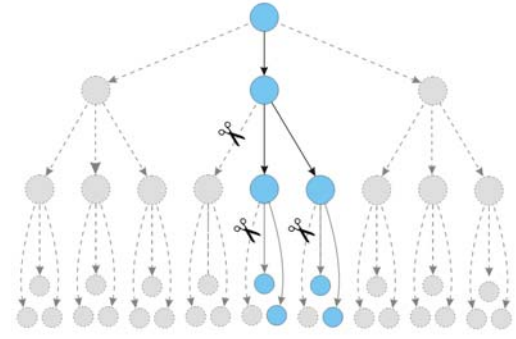
Figure 57. Effect of dynamic relevance estimation on the overall search space, assuming 33% of nodes are filtered.
