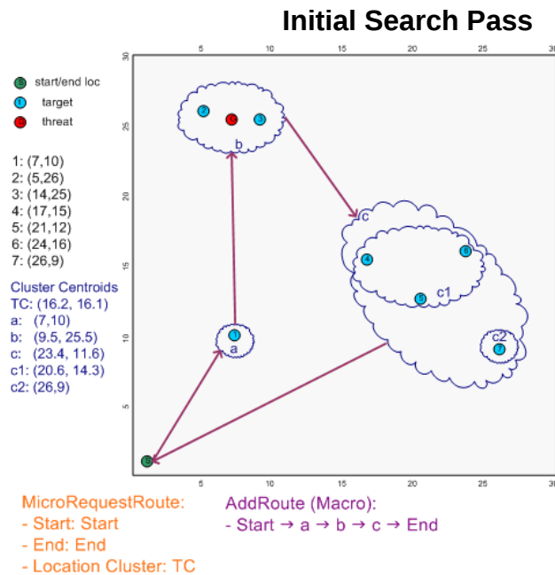
Figure 44. Micro attempts to construct a coarse route sequencing the clusters themselves. For expository purposes, in this example Micro is unable to find a route in its store of experience, so it asks Macro to construct a fresh route. Micro learns the route and will be able to reuse it in future cases.
