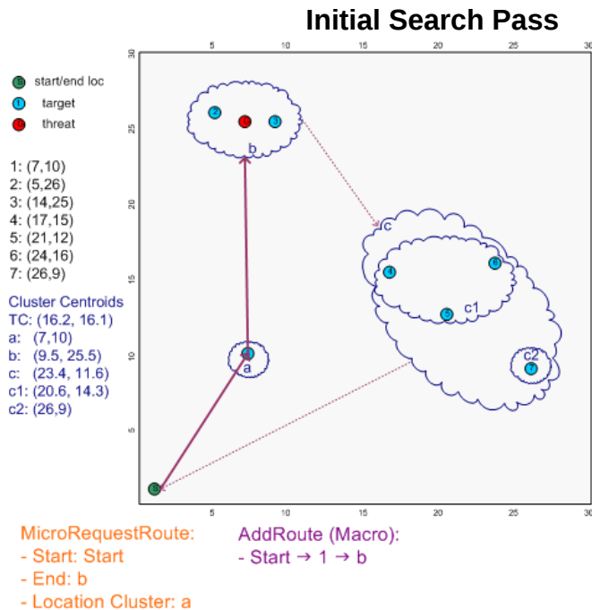
Figure 45. Having a top-level route, Micro must now delve into the clusters, forming intra-cluster routes. The first cluster is trivial, containing only one target.
