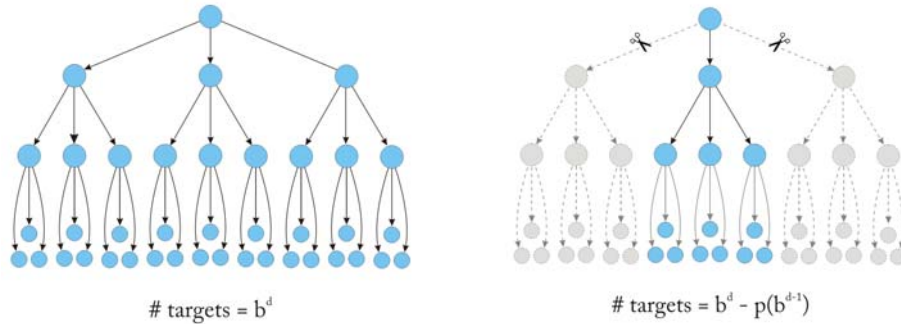
Figure 56. Simple illustration of the size of a search space (left) and the effect of attentional filtering (right).
