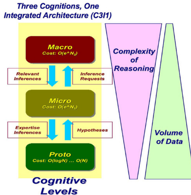
Figure 1. PCAA cognitive approach and the cognitive components
