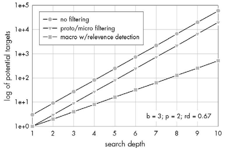
Figure 58. Search depth vs. log of potential targets for hypothetical problem in which branching factor =3, filtering effect is 2, and relevance estimation removes 33% of available options.
