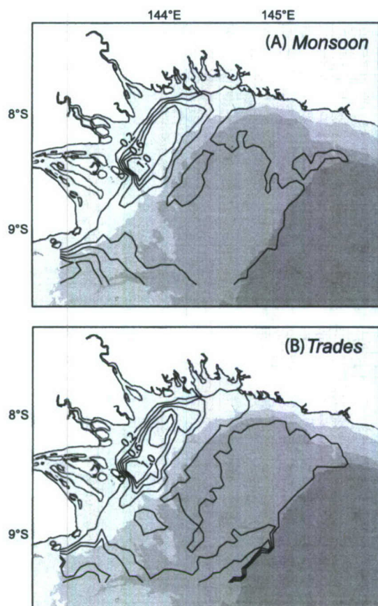
Figure 13. Maximum bed layer shear stress due to currents (Pa) predicted by NCOM over a lunar cycle during (a) monsoon and (b) trade wind seasons. Contour interval is 0.2 Pa. Shear stresses computed as \rho f U^2 where \rho = 1025 \text{ kg m}^{-3} , Darcy-Weisbach friction factor, f = 0.0025 , and U is the largest current magnitude at a site over a lunar cycle. Bathymetry from light to dark gray in increments of -20 , 20-60 , 60-160 , and >160 m. Note that maximum bed shear stresses are dictated mainly by tides and therefore show little variation between the two seasons.
