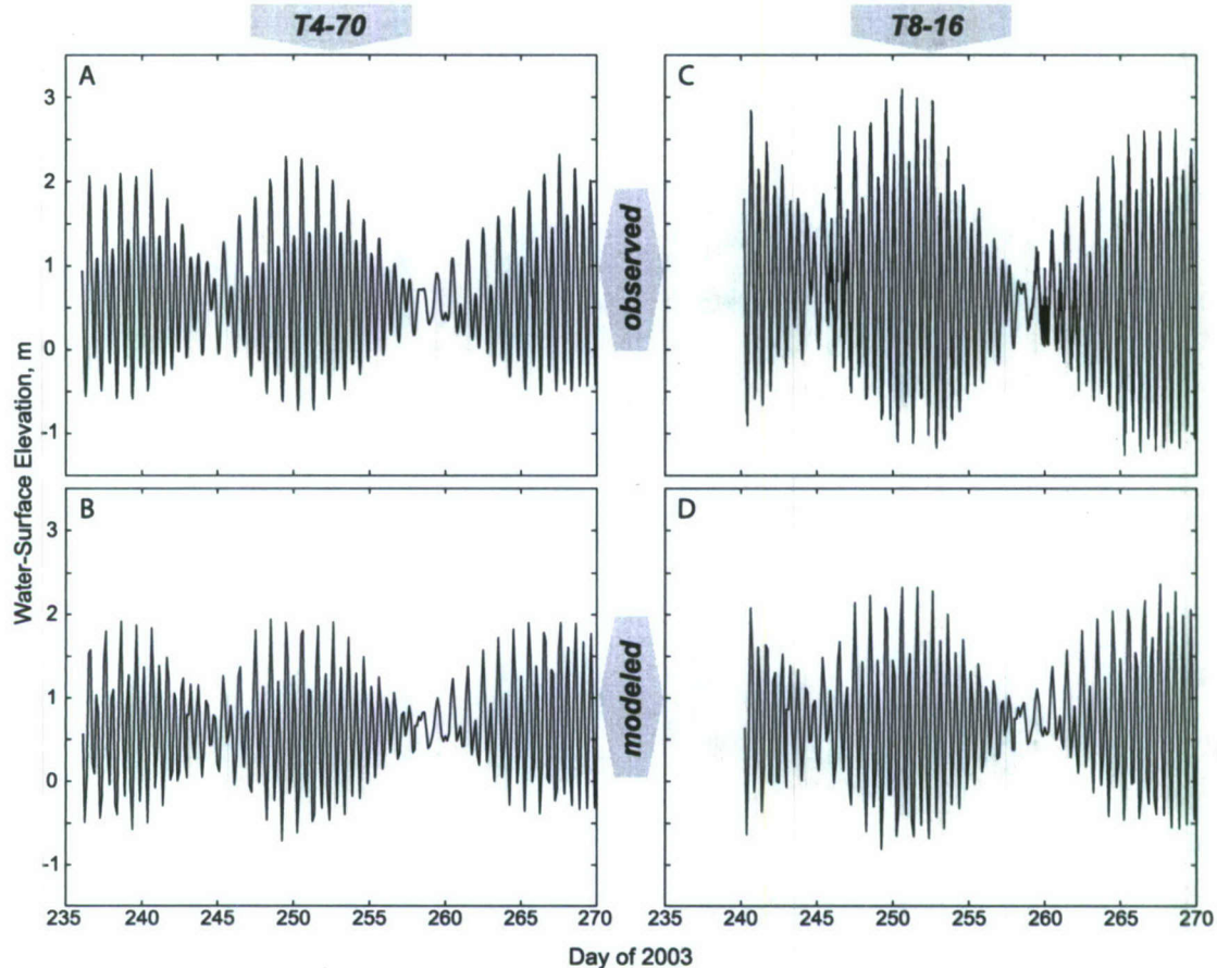
Figure 3. Observed and modeled water surface elevations from 25 August to 25 September 2003 at observation locations and nearest NCOM grid node (a) observed at T4-70 ( 9^{\circ}07.482' , 144^{\circ}24.545' ), (b) modeled at NCOM node nearest T4-70, (c) observed at T8-16 ( 8^{\circ}34.535' , 143^{\circ}57.817' ), and (d) modeled at NCOM node nearest T8-16.
