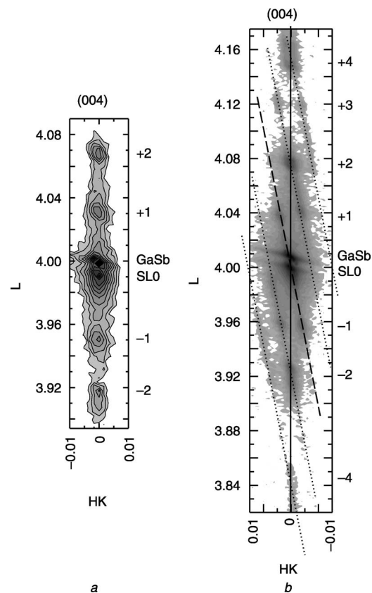
Fig. 3 XRD reciprocal space map of LCM in 140 period \text{InAs}/\text{GaSb} superlattice about (004) Bragg peak with \Phi = 0^\circ (a) and \Phi = 90^\circ (b)
