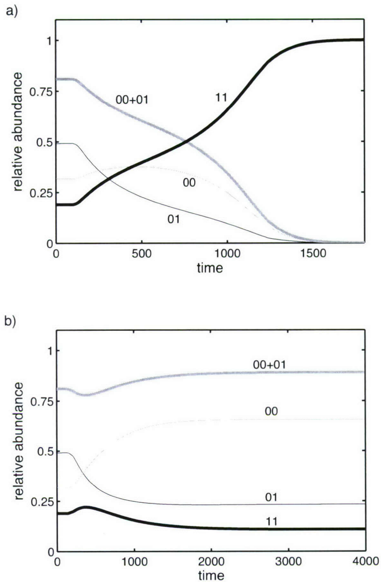
Figure 2-8: Frequency of zooplankton types versus time, for two different values of the parameter \tau , with S = 5 . a) \tau = 0.04 , the grouping type (11, thick black curve) outcompetes the resident population (00+01, thick gray curve). b) \tau = 0.1 , the grouping type aggregates but does not invade the resident population. Decreasing \tau has the effect of accelerating mixing relative to predation, thus effectively increasing resource supply to clustered zooplankton. Initially the grouping type represents a fraction f_c of the population.
