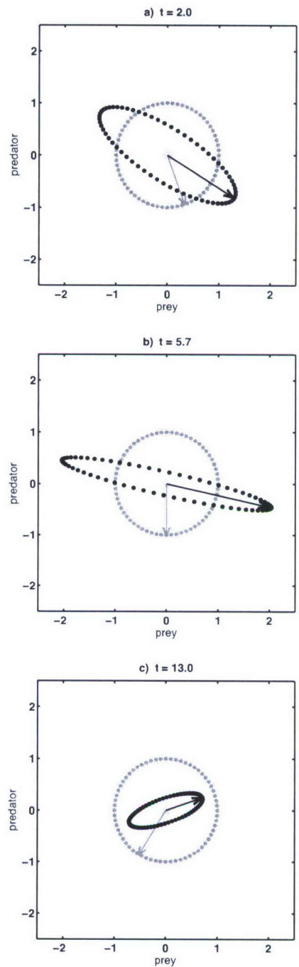
Figure 5-1: Transient amplification of perturbations in the predator-prey model (5.54–5.55) at t = 2.0 (showing growth of perturbations), t = 5.7 (maximum of the amplification envelope), and t = 13 (as perturbations decay). Initial conditions (with unit norm) are represented by gray dots; the response is shown by black dots. Parameters from Table 5.1, Equilibrium A.
