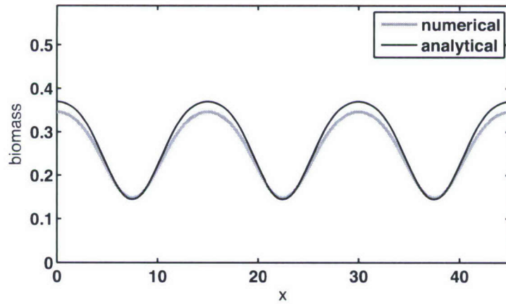
Figure 3-4: Steady-state solution to the weakly nonlinear equations (black line) and fully developed patches in the numerical model (gray line); the system is initially perturbed at a single wavenumber ( k = 0.42 ). \mathcal{S} = 2 ; other parameters as in Figure 3-1.
