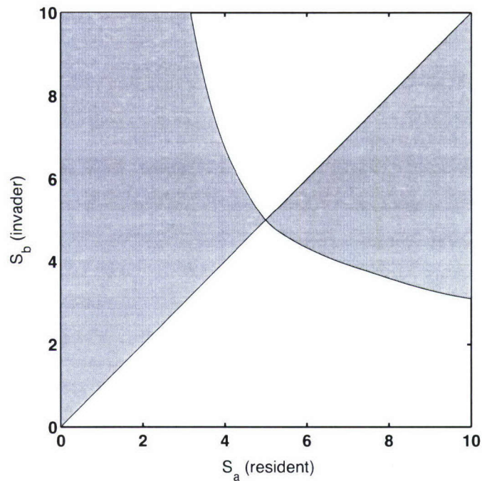
Figure 3-9: Pair-wise competition diagram; gray shading indicates that type b (y-axis) outcompetes type a (x-axis). S = 5 is optimal. Parameters as in Figure 3-8.
