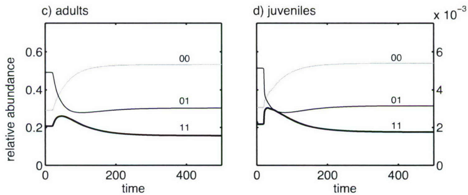
Figure 2-11: Relative abundance of zooplankton versus time in the structured model, for slow recruitment (top) and fast recruitment (bottom). a) and b) q = 1 : the grouping type (11, thick black curve) outcompetes the resident population (00+01, thin curves); the frequency of the grouping allele increases monotonically in the juvenile and adult populations. c) and d) q = 100 : the grouping type does not invade the resident population. When recruitment is fast, juveniles are a negligible fraction of the total population so that the model is equivalent to an unstructured predator-prey model.
