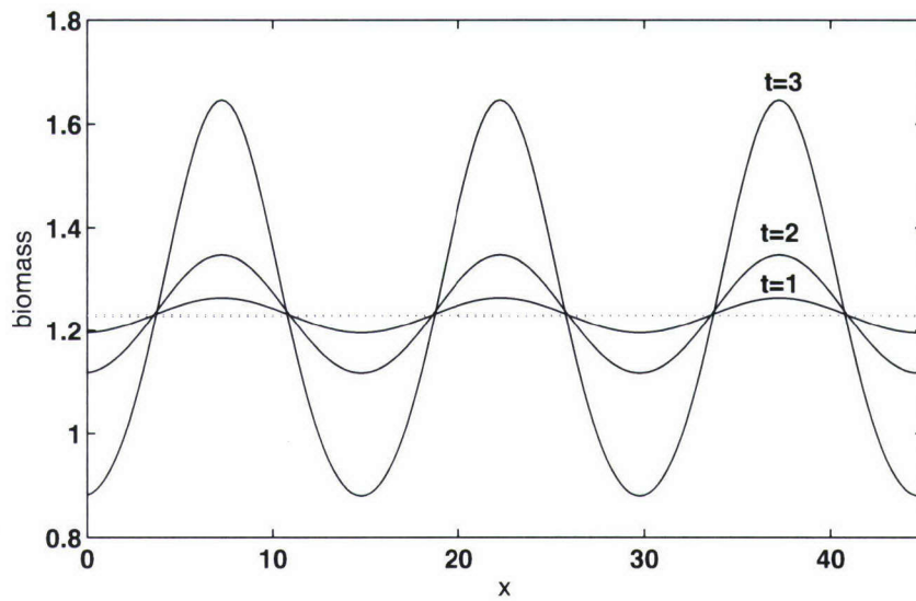
Figure 3-1: Initial growth of patches in the predator distribution. Parameters are \mathcal{S} = 2 , \nu = 10 , \gamma = \lambda = 1 , \chi = 0.5 , \delta = 0.1 ; the weighting function is W = e^{-x^2/2} - 1.2e^{-x^2} . The scale of patchiness is determined by the mode with the largest growth rate. Dotted line indicates mean biomass.
