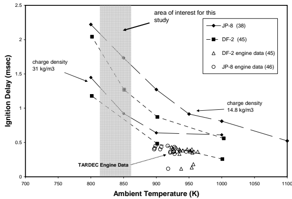
Figure 4: Comparison of DF-2 and JP-8 Ignition Data at Various Ambient (Charge) Densities. Cetane number for each fuel is given in parenthesis within the legend.
