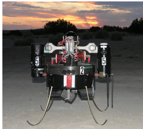
Figure 2. MAV Vehicle
