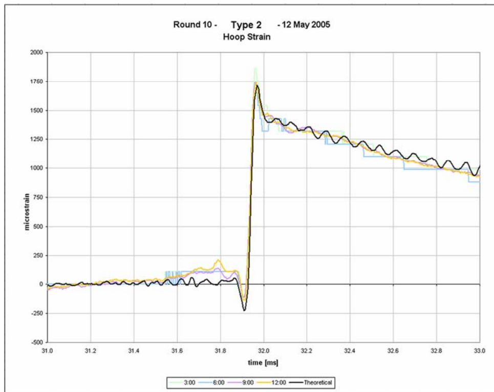
Figure 7—Experimental & theoretical strain vs. time
