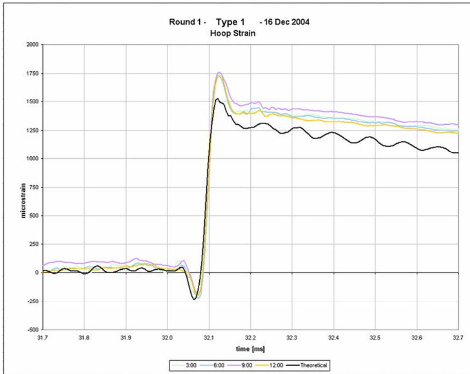
Figure 6—Experimental & theoretical Strain vs. time
