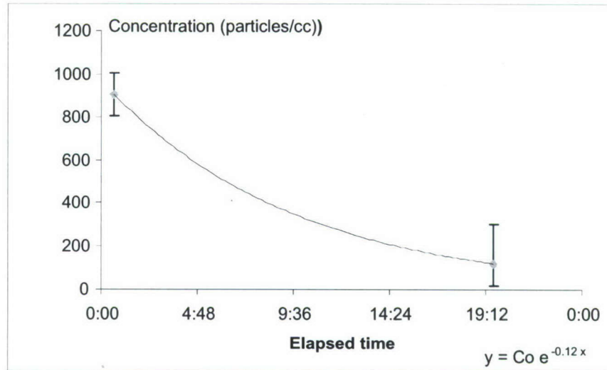
Figure 6. Concentration Decay Overnight inside the Modified Chamber. C_f = C_0[e^{-0.12 x}]
