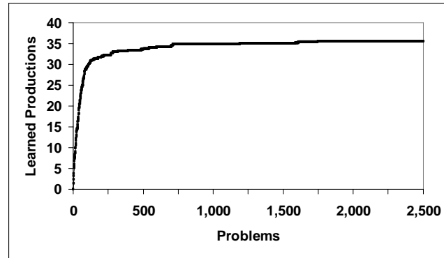
Figure 3: Productions Learned in ACT-R
