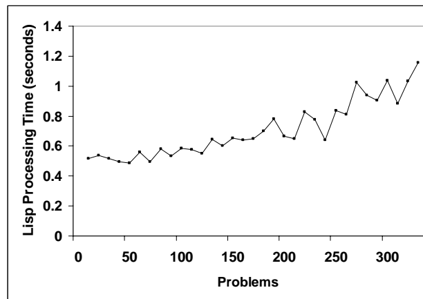
Figure 6. ACT-R Run Times for Blocks-World Problems
