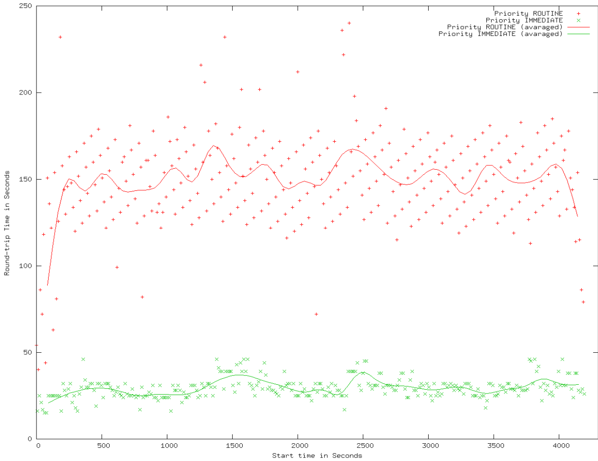
Figure 8: Two priorities with 1200 bits/sec FLASH voice background
