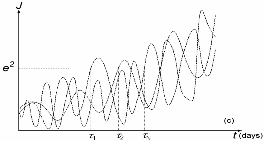
Fig. 1 The IPT and e-folding time for an oscillating prediction error. (a) IPT ( \tau ) computed in an individual forecast. Shaded zones show returns of model predictability. (b) an ensemble of J (dashed curves), the ensemble averaged J (solid curve) and the e-folding time ( \tau_e ), and (c) the ensemble of J (dashed curves) and an appropriate ensemble of IPT( \tau_1, \dots, \tau_N ).
