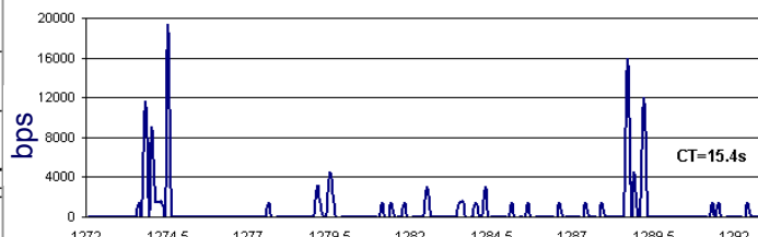
Network convergence time after NE's disconnection from the network [seconds]
