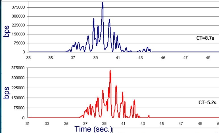
Network convergence time after NE's reconnection to the network [seconds]
