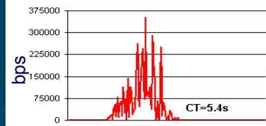
Network convergence time after NE's reconnection to the network [seconds]
