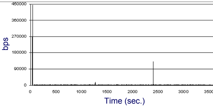
Total amount of BGP routing information sent after NE's dislocation (bps)
