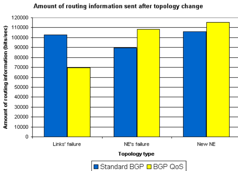
Figure 11. Routing information amount comparison.
