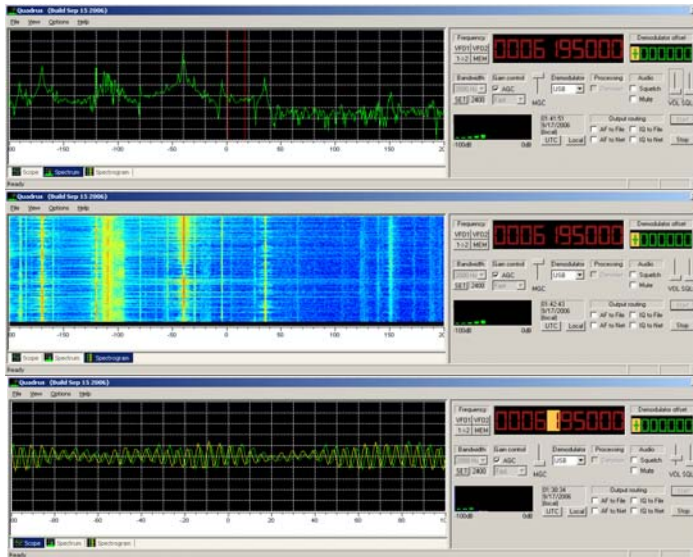
Figure 17: Monitoring receiver
