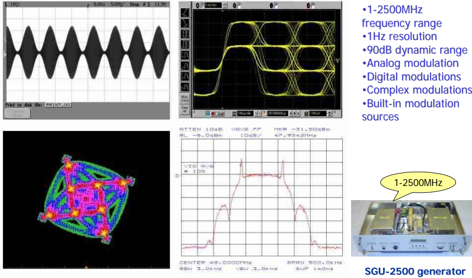
Figure 15: Modulation generator
