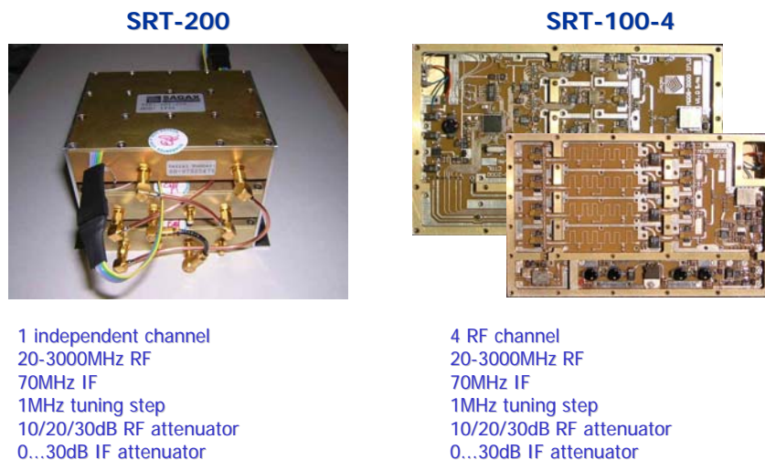
Figure 8: RF front-ends
