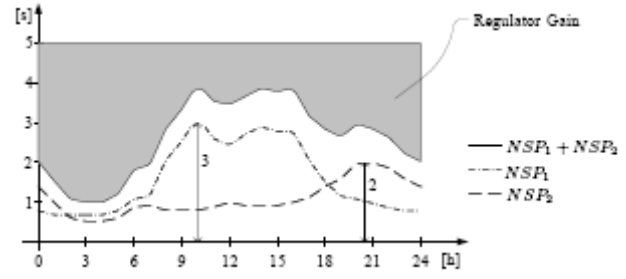
Figure 3: TDSA Regulator Gain
