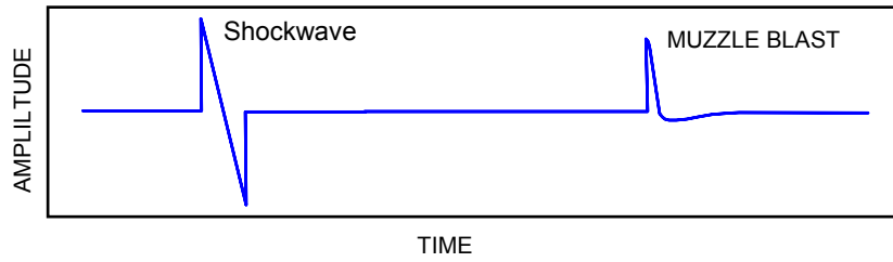
Figure 3: Idealized sound received at a microphone exposed to small arms fire (U)
