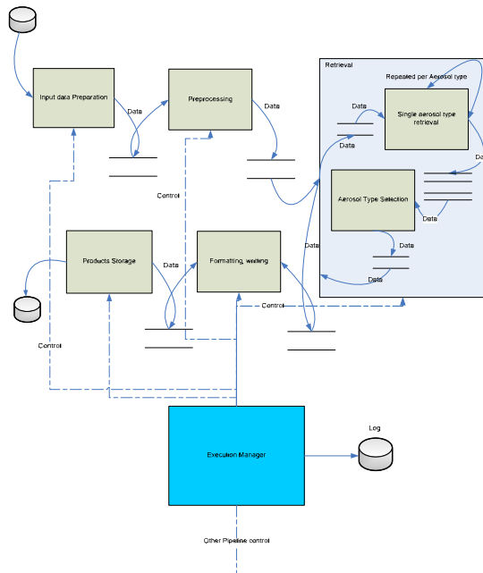
Figure 5 GlobAEROSOL Architecture
