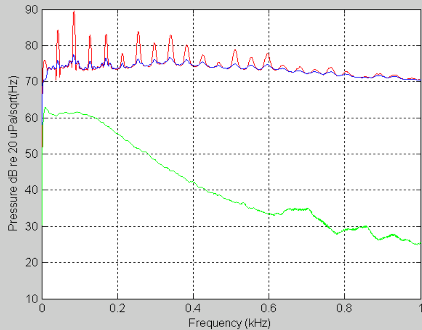
TUAV In Flight
