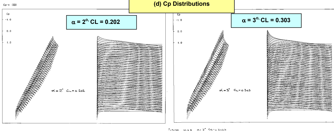
Fig. 7 30° OFW ISOLATED PLANAR CASE Mach 0.8, AoA Effects
