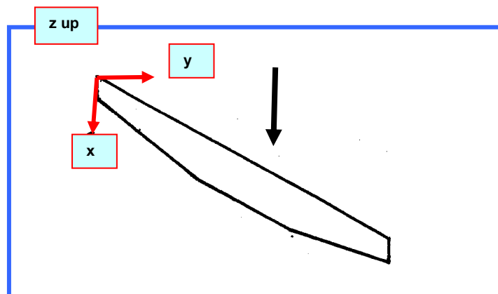
Fig. 6 OBLIQUE FLYING WINGS, PLAN GEOMETRY ASSUMED, 30 deg. LE SWEEP
