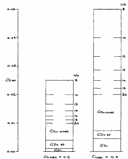
FIG. 28 TOTAL DRAG BREAKDOWN, C_{Di} , C_{DSF} , & C_{Dothor} CONTRIBUTIONS FOR VARYING L/D AT Mach 0.8, CL_{des} = 0.2 & 0.4
