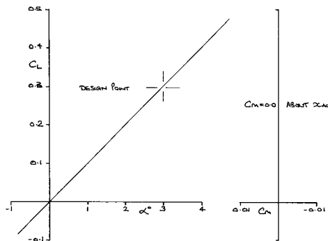
(a) Lift &amp; Pitching Moment
