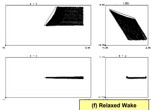
Fig. 8 30° OFW ISOLATED DESIGN CASE No C_{LL} constraint, Mach 0.8, C_L=0.3
