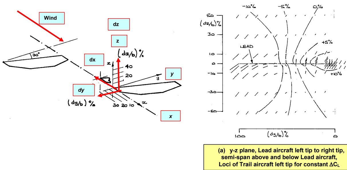
Fig. 15 CORE 1 FORMATION DISPLACEMENTS, GEOMETRY DEFINITIONS
