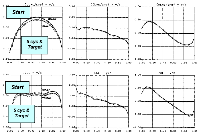
(b) Spanwise Loadings at Start &amp; after 5 cycles
