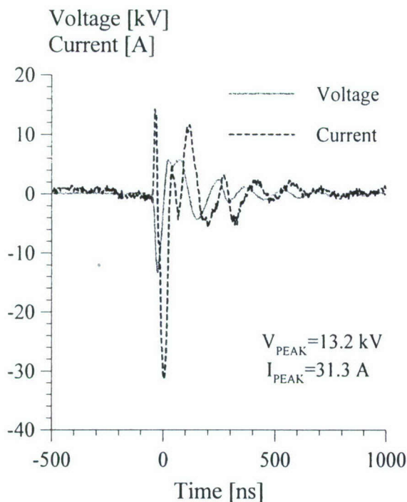
Figure 3. Single-pulse voltage and current oscillograms in a M=3 nitrogen flow at P_0=250 torr, P_{test}=8.4 torr, and B=1.5 T.
