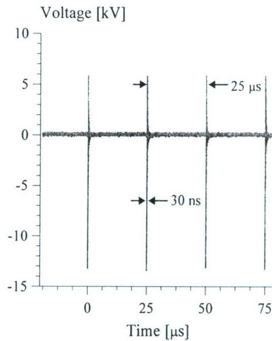
Figure 2. Typical repetitively pulsed voltage waveform. M=3 nitrogen flow at P_0=250 torr, P_{\text{test}}=8.4 torr, and B=1.5 T [12]. Pulse repetition rate is \nu=40 kHz.
