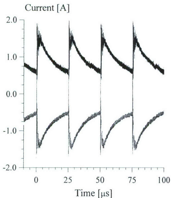
Figure 5. Sustainer (Faraday) current traces for two different transverse DC electric field polarities, at the conditions of Fig. 4. U_{PS}=2 kV, R=0.5 k \Omega . Time-averaged currents are 0.95 A (top curve) and 0.86 A (bottom curve).
