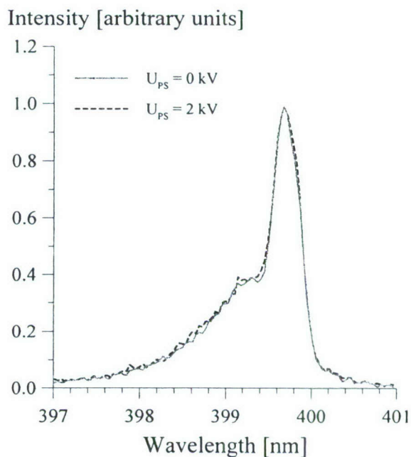
Figure 6. N_2(C3\Pi_u \rightarrow B^3\Pi_g) emission spectra (1 \rightarrow 4 band) in a M=3 nitrogen flow at P_0=250 torr, B=1.5 T, and \nu=40 kHz, with and without 1.4 kW DC sustainer discharge. Synthetic spectrum fit indicates rotational temperature of T=180 \pm 20 K in both cases.
