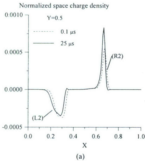
Figure 15. Instantaneous normalized space charge density at two different moments of time (a) and ion slip velocity predicted by Eq. (19) (b) at Y=0.5 . Conditions are the same as in Figs. 11, 12.
