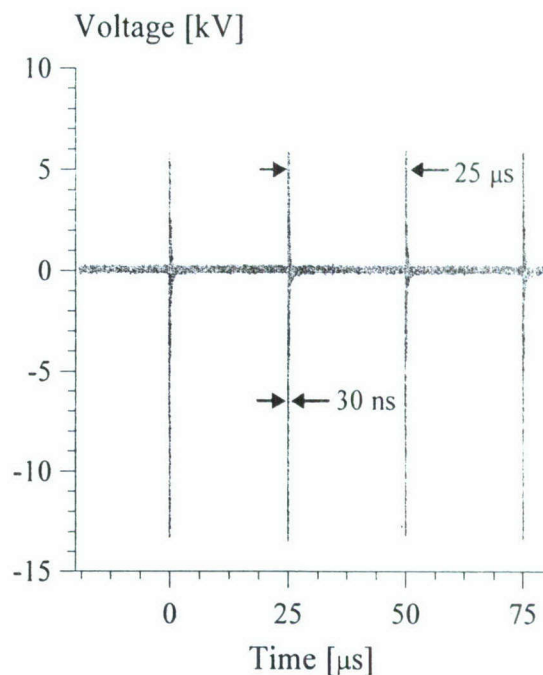
Figure 4. Repetitively pulsed voltage oscillogram in a M=3 nitrogen flow at P_0=250 torr, P_{test}=8.4 torr, and B=1.5 T. Pulse repetition rate is \nu=40 kHz.
