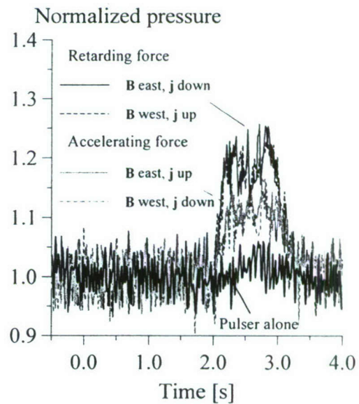
Figure 13. Normalized static pressure traces in a M=4 nitrogen flow at P_0=600 torr, P_{test}=4.8 torr, B=1.63 T, \nu=100 kHz. U_{PS}=1.4 kV, and R=0.5 k \Omega . Lorentz force is applied for 1 sec duration.
