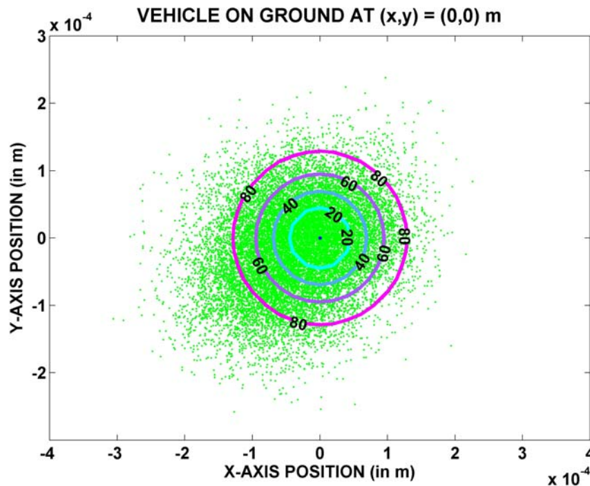
Figure 3: X-Y Scatter plot of 7 mins of measured (x, y) vehicle position at 50 Hz – rotors not turning. Note that the scale in these plots is meters \times 10^{-4} . The circles in this plot designate the percentage of the data points from (x,y) = (0,0) m. Note that over 80% of the points are within 0.00015 m of (x,y) = (0,0) m.
