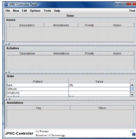
Figure 37: Initial state of the JPRC controller’s I-X Process Panel
