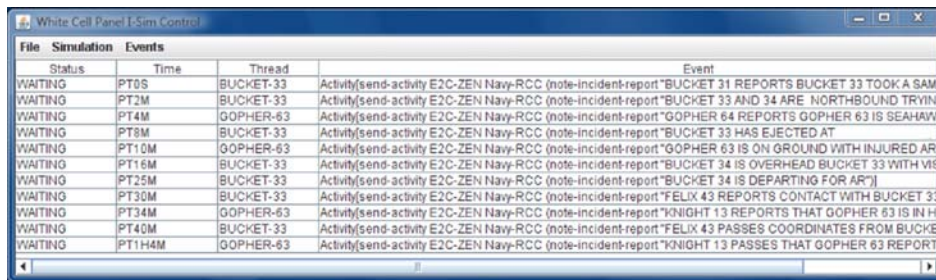
Figure 18: The I-Sim Tool for controlling the events that will occur
