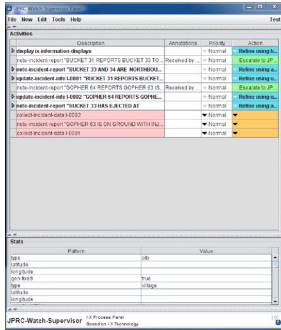
Figure 31: The Watch Supervisor's Panel (2)
