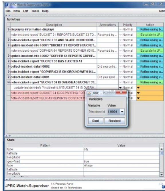
Figure 34: The Watch Supervisor's Panel (5)
