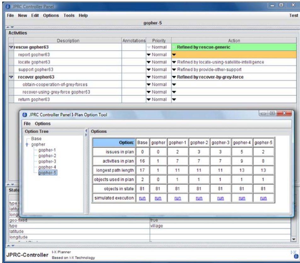
Figure 46: Using the I-Plan Option tool to compare options
