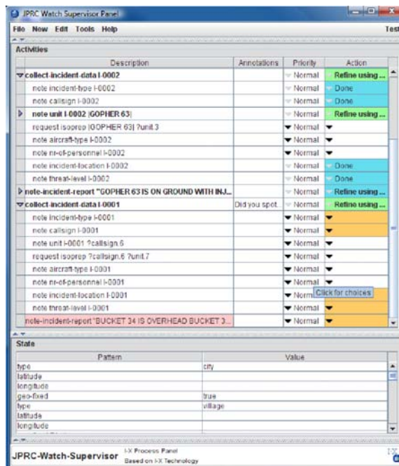
Figure 32: The Watch Supervisor's Panel (3)
