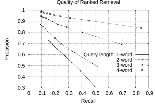
Figure 7: Performance on ranked retrieval with different query sizes.
