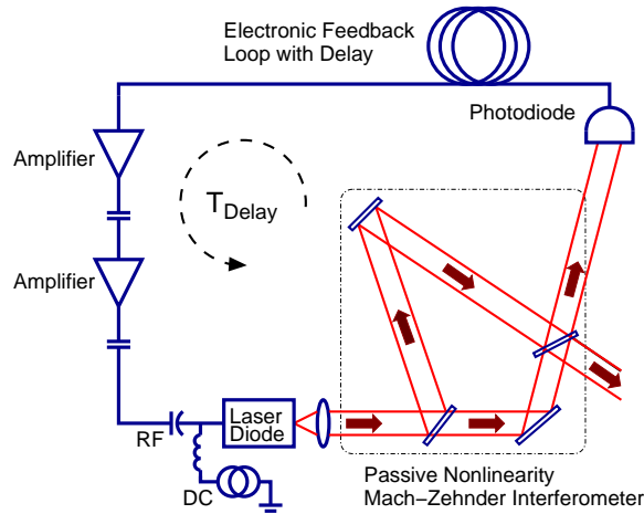
Figure 1. Schematic of experimental setup. The device consists of a voltage controlled source, a passive nonlinearity, and a feedback loop with bandpass characteristics. Details of the setup are explained in the text.
