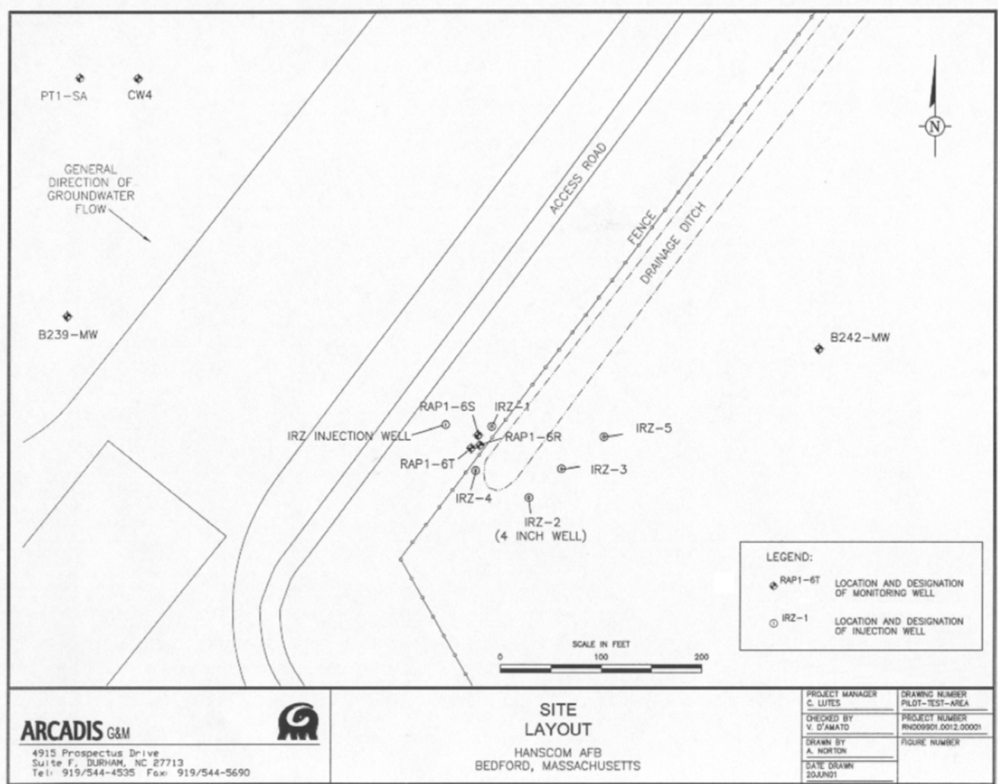
Figure 6. Hanscom AFB Site Layout, Pilot Test Area
