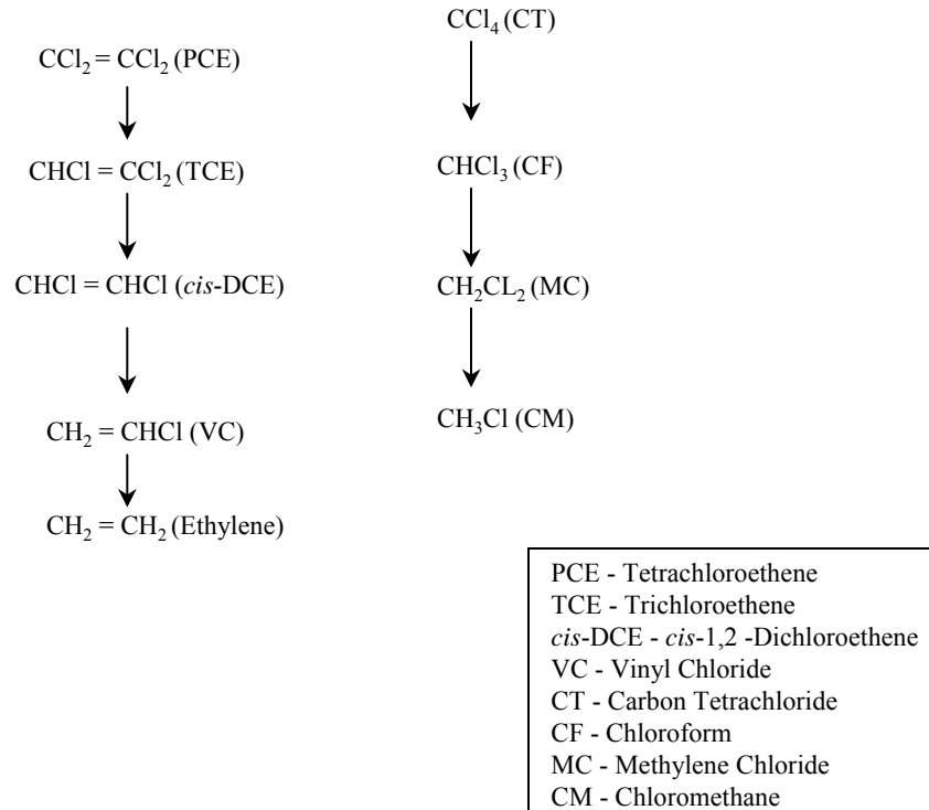
Figure 1. Anaerobic Transformations of Selected CAHs and Their Daughter Products (Vogel et al, 1987 and McCarty and Semprini, 1993).
