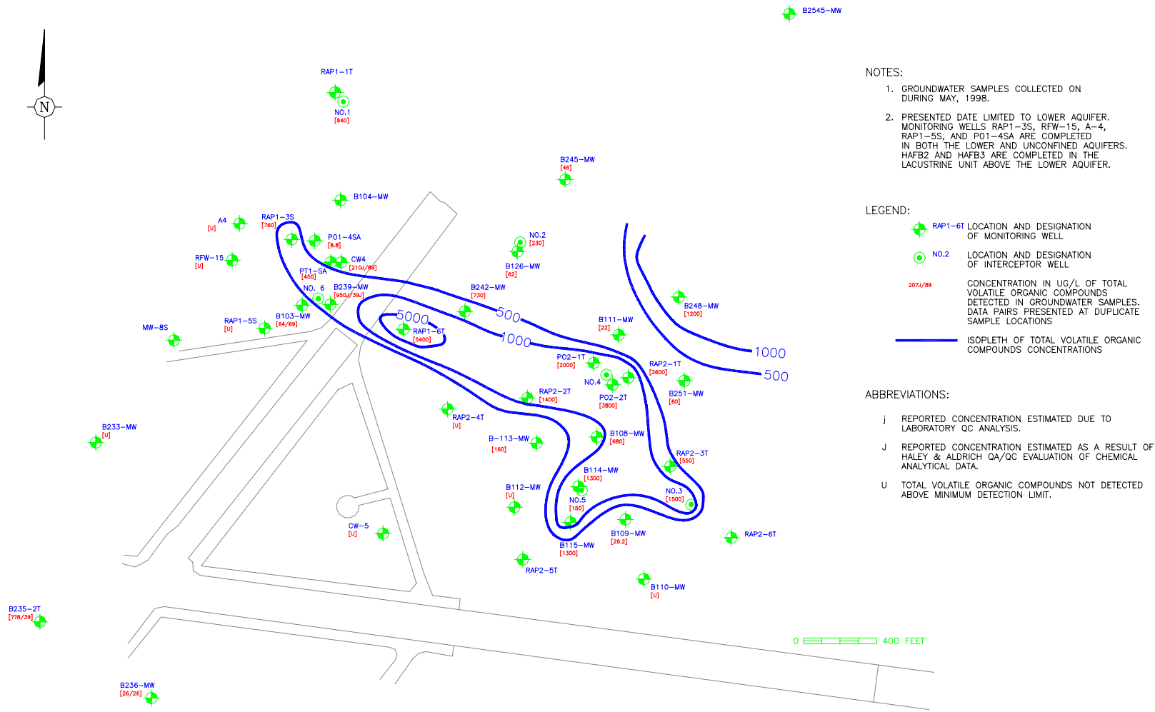
Figure 5. Total Volatile Organic Compound (VOC) Concentrations in Lower Aquifer Near RAP1-6T, May 1998—HAFB
