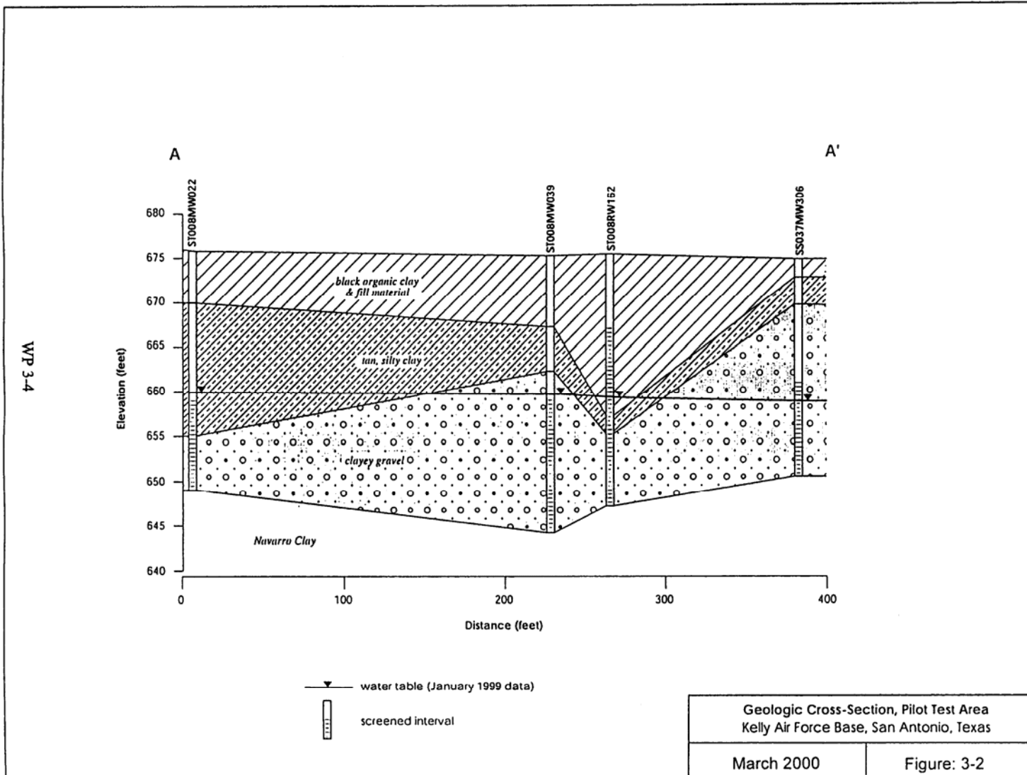
Figure 1. Cross-Sectional Diagram of the Surface Geology at Site 360, Kelly AFB.
