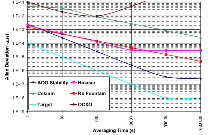
Fig. 2. Comparison of frequency stability in various devices at 5 MHz assuming a system bandwidth of 1 MHz
