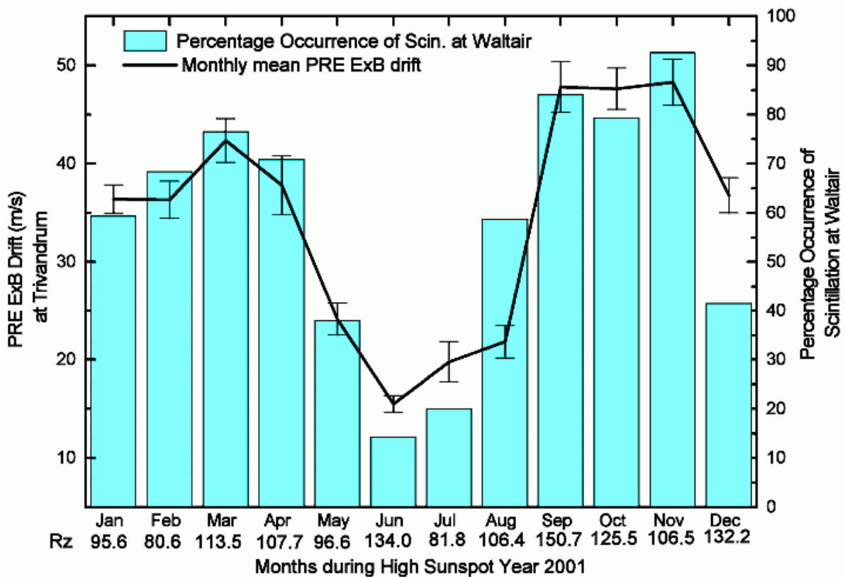
Fig 8. The correspondence between the monthly mean PRE ExB peak drift velocities (solid line) and percentage occurrence of VHF scintillations (vertical bars) during a high sunspot year 2001.
