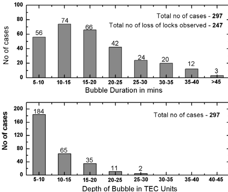
Figure 6. Statistics showing the duration (a) and intensity (b) of the TEC depletions observed over Indian region for the month of March 2004.
