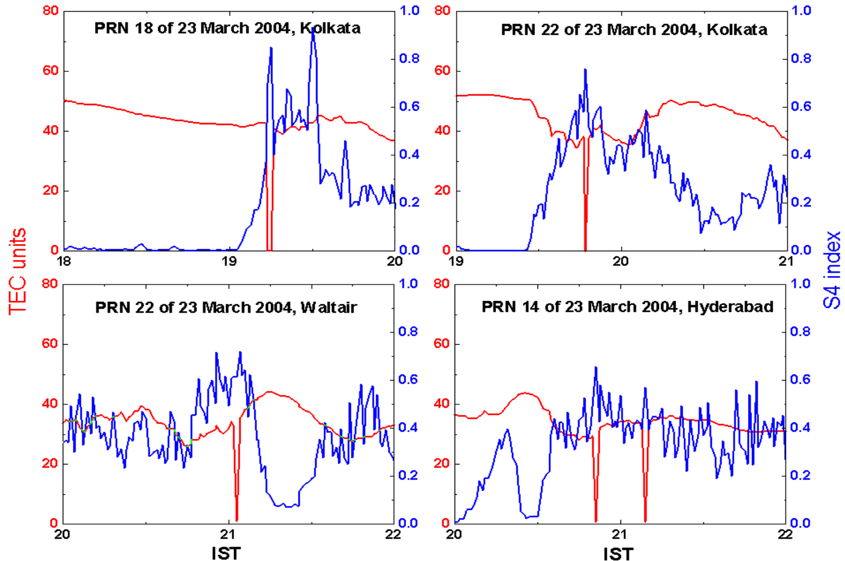
Typical Examples of the loss of lock of the GPS receivers
