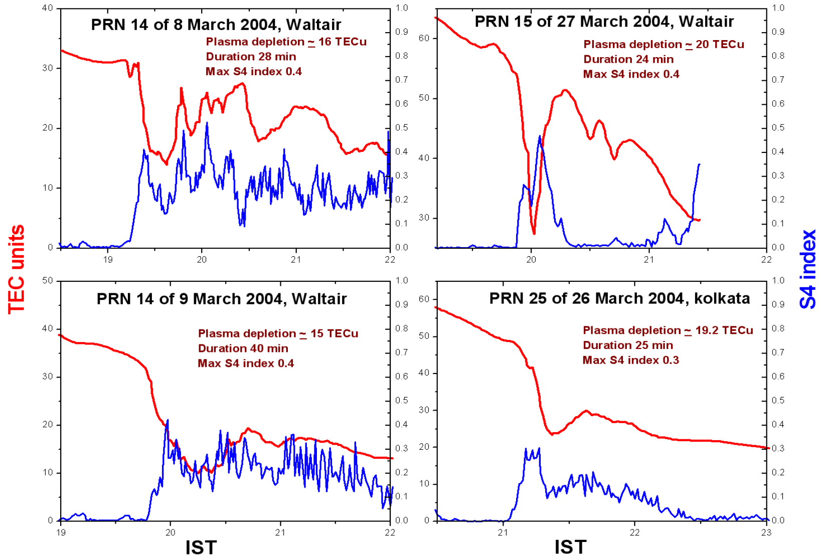
Typical examples of TEC depletions observed and the corresponding S4 index variations
