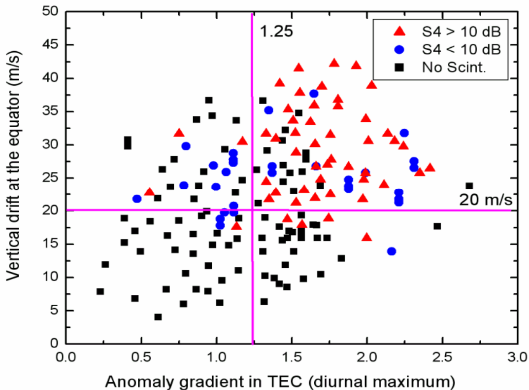
Fig. 14: Post sunset vertical drifts at the equator as a function of peak anomaly gradient in TEC (diurnal maximum) for each day during 2004. The red triangles indicate the strong scintillation ( \geq 10 dB) days, blue circles indicate weak scintillation ( < 10 dB) days and black squares indicate the days on which no significant scintillations were observed at GPS L1 frequency.
