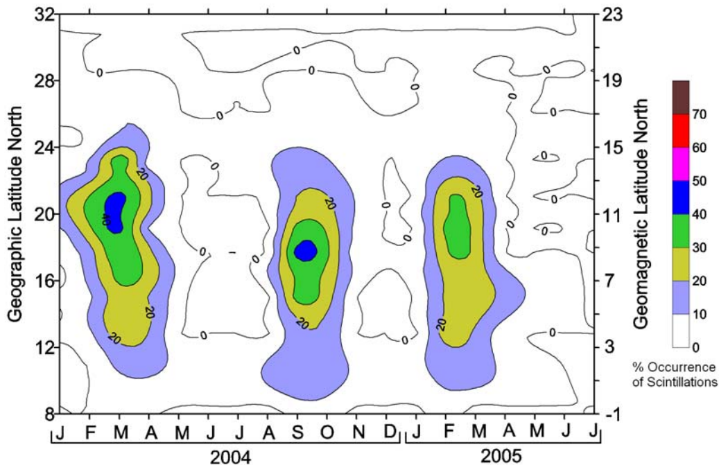
Figure 3. Temporal & Spatial variation in the Occurrence of scintillations > 10 dB power levels during the low sunspot activity years of 2004 and 2005.
