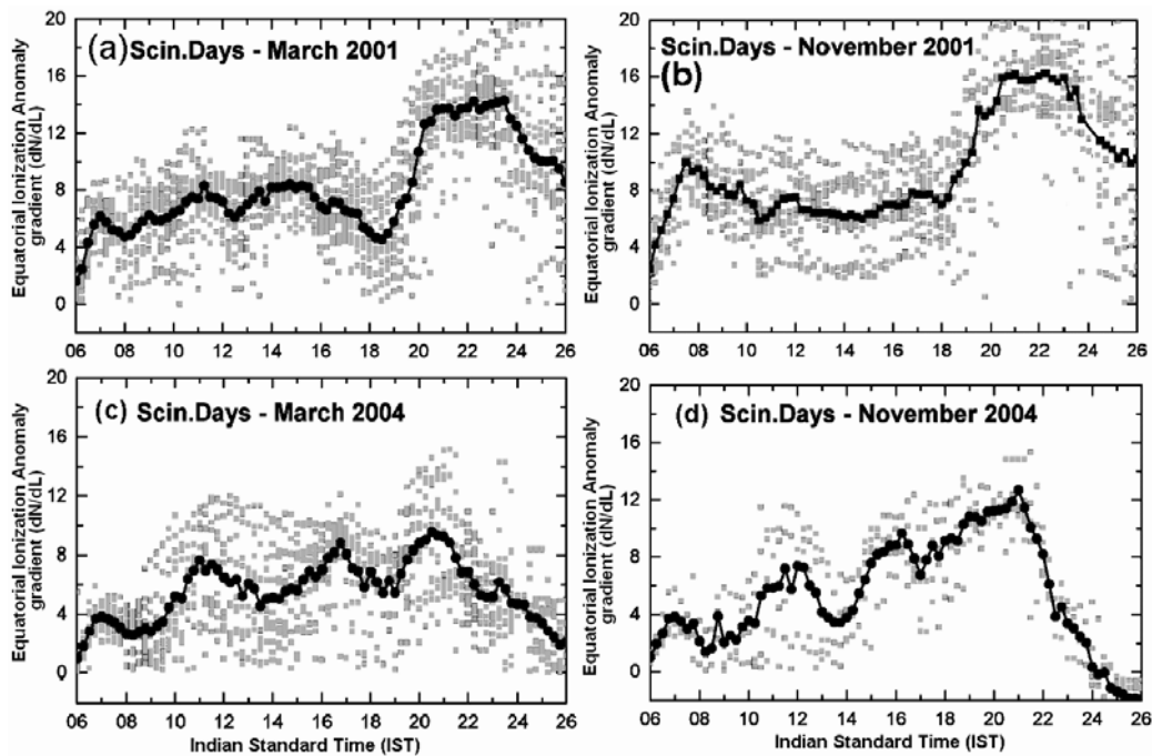
Fig. 10: The diurnal variations of the Equatorial Ionization Anomaly gradients (dN/dL) for the days on which strong ( \geq 10 dB) scintillations have occurred during (a) March 2001, (b) November 2001, (c) March 2004 and (d) November 2004.
