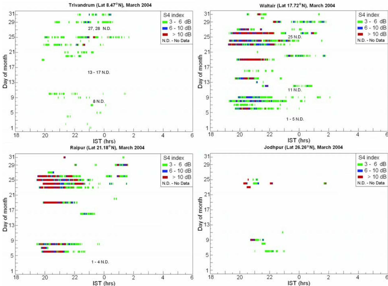
Figure 2. Day to Day occurrence of scintillations with different power levels for the month of March 2004 for four typical Indian latitudes representing (a) Equatorial station (Trivandrum), (b) low latitude station (Waltair), (c) anomaly crest station (Raipur), (d) station beyond the anomaly crest (Jodhpur)
