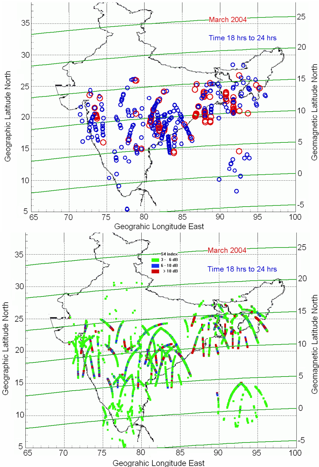
Figure 5. Occurrence of L-band scintillations associated with TEC depletions (bubbles) and loss of lock events during the month of March 2004. (a) Bubbles (blue circles) and loss of locks of the GPS receivers (red circles) and (b) The scintillations at three different power ranges of 3 to 6 dB (Green), 6 to 10 dB (Blue) and > 10 dB (Red).
