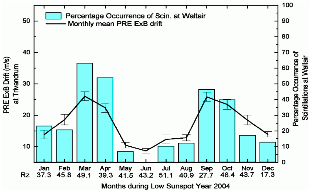
Fig. 9: The correspondence between the monthly mean PRE ExB peak drift velocities (solid line) and percentage occurrence of VHF scintillations (vertical bars) during a low sunspot year 2004.
