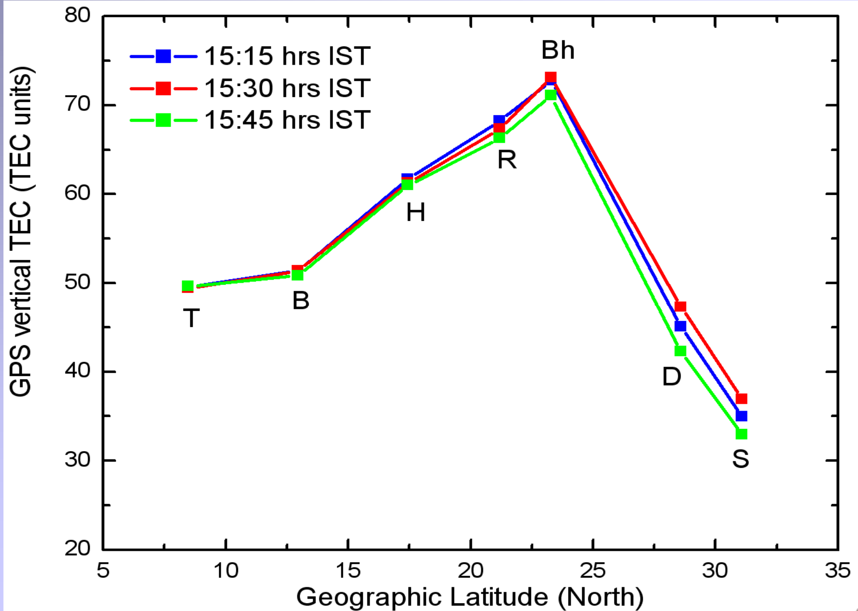
TEC values at the seven stations along the common meridian
