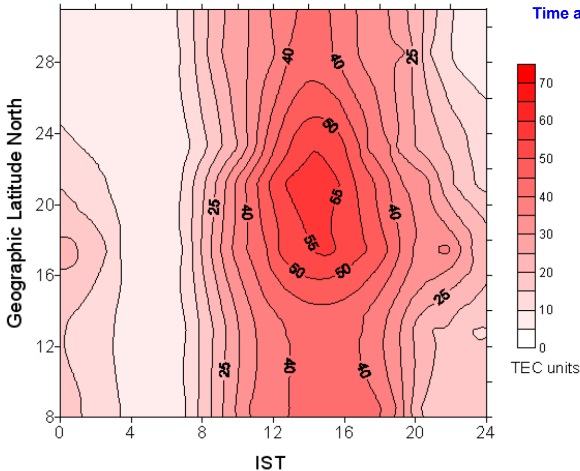
Monthly average diurnal variation of TEC for the month of MARCH 2004.
