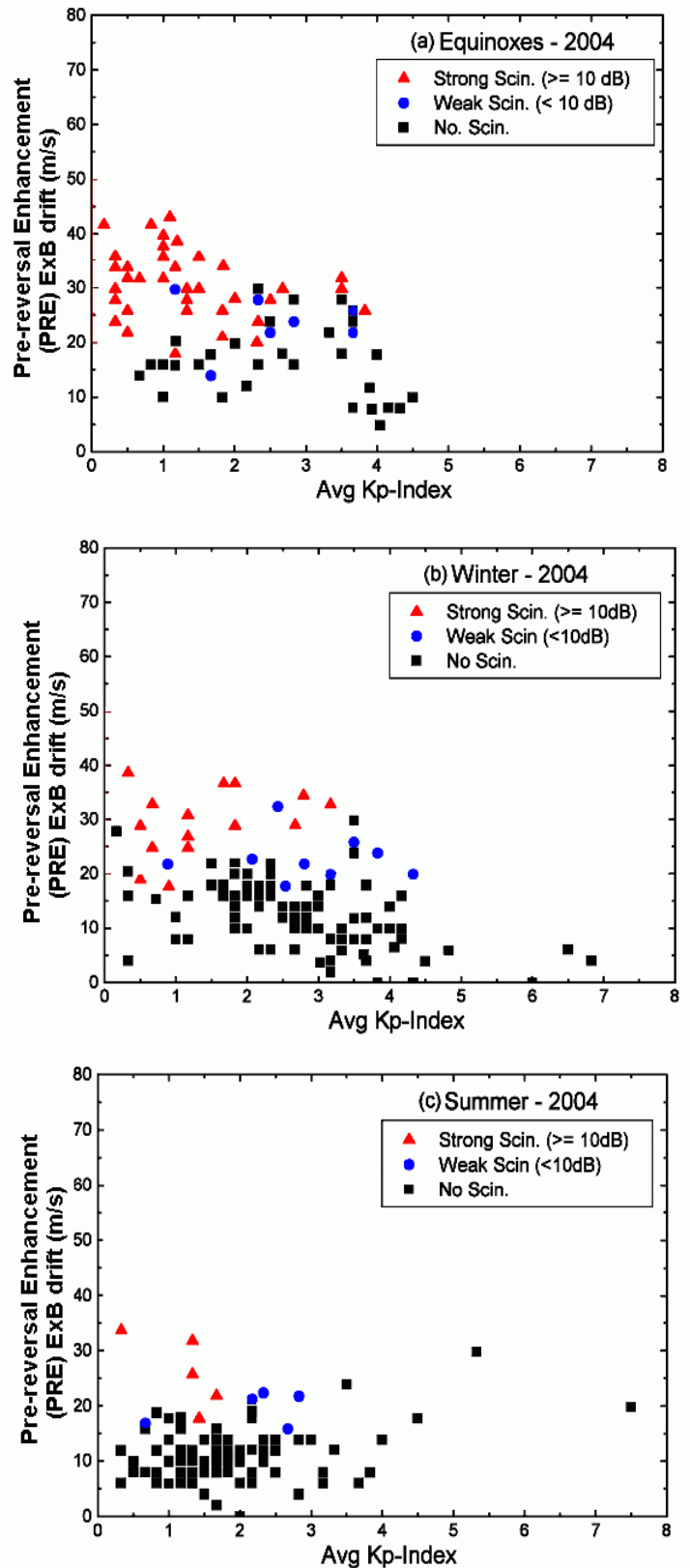
Fig. 13 : The Pre-reversal enhancement (PRE) ExB drift velocities as a function of the 6-hour average Kp, observed for each day during (a) equinoxes, (b) winter and (c) summer months of low sunspot activity year, 2004.
