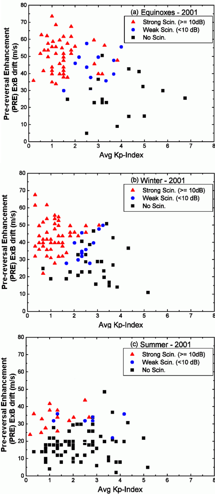
Fig. 12 : The Pre-reversal enhancement (PRE) ExB drift velocities as a function of the 6-hour average Kp, observed for each day during (a) equinoxes, (b) winter and (c) summer months of high sunspot activity year, 2001.
