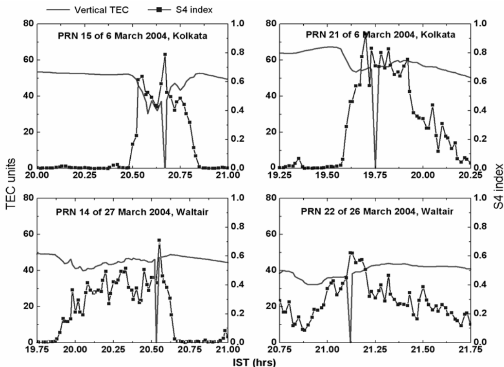
Figure 7. Typical examples of scintillation activity showing the values of S4 index exceeding 0.45 causing loss of lock of the GPS receivers.
