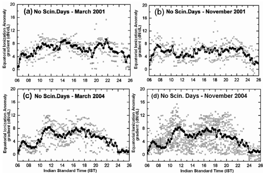
Fig. 11: The diurnal variations of the Equatorial Ionization Anomaly gradients (dN/dL) for the days on which scintillations are weak ( < 10 dB) or absent during (a) March 2001, (b) November 2001, (c) March 2004 and (d) November 2004.
