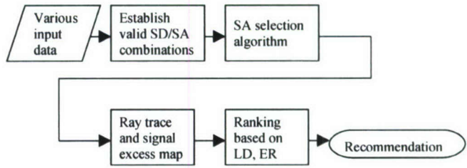
Fig. 3. Flow chart for illustrating the WAPP presetting procedure.
