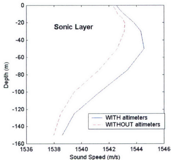
Fig. 16. Comparison of MODAS SSP at 32.5^{\circ} N, 127.5^{\circ} E on October 10, 2001 with and without satellite altimetry data assimilated. Note the existence of a sonic layer.
