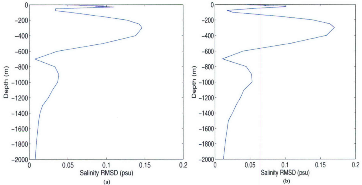
Fig. 7. Horizontal RMSD of MODAS salinity for KCA on (a) June 30, 2001 and (b) October 10, 2001.
