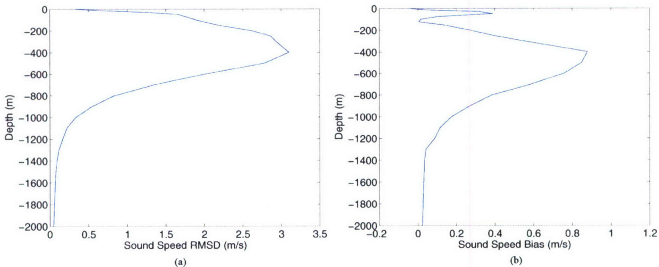
Fig. 13. (a) Horizontal RMSD and (b) bias of MODAS SSP for KCA on June 30, 2001.
