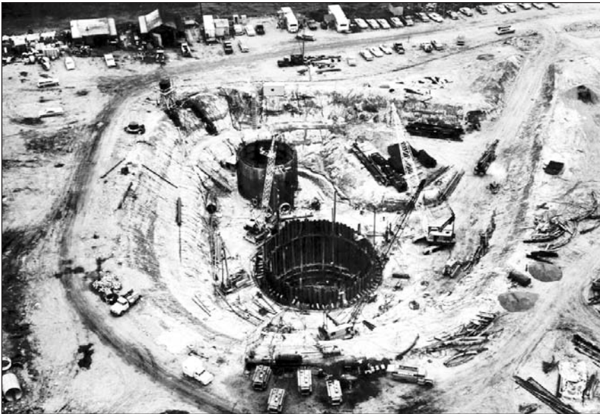
Construction site, early 1960s, for the Series F Atlas ICBM “silo-lift” launcher at Plattsburgh Air Force Base, New York. On a “silo-lift” launcher, the missile is stored vertically within a hardened, underground silo.
