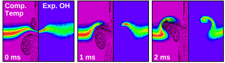
Figure 1. Computed temperature vs. OH PLIF data for a flat counterflow diffusion flame perturbed by multiple vortices.
