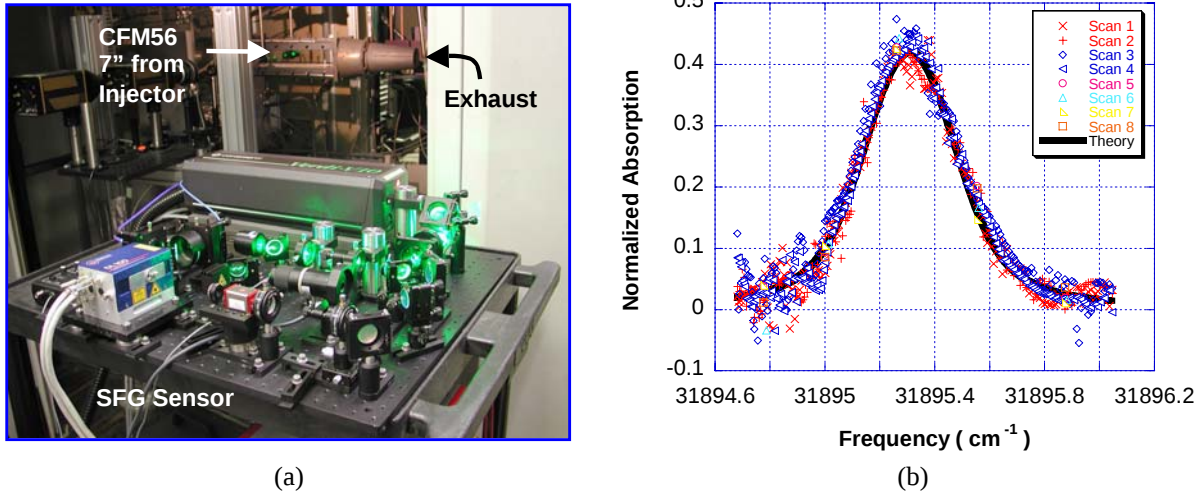
Figure 1. (a) High-speed OH sensor in CFM56 facility and (b) theoretical fit to multiple OH spectral scans at 20 kHz in CFM56 flame zone.
