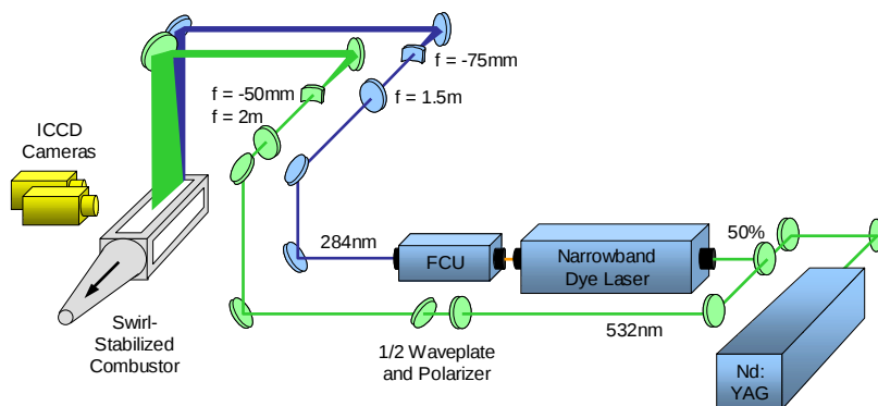
Fig. 1. Simultaneous OH PLIF and LII in atmospheric-pressure, swirl-stabilized, JP8-fueled, model gas-turbine combustor.
