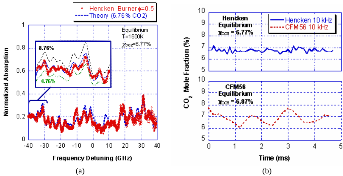
Figure 2. (a) Validation of \text{CO}_2 theoretical model in Hencken burner and (b) 10-kHz \text{CO}_2 time series in exhaust of CFM56 combustor.
